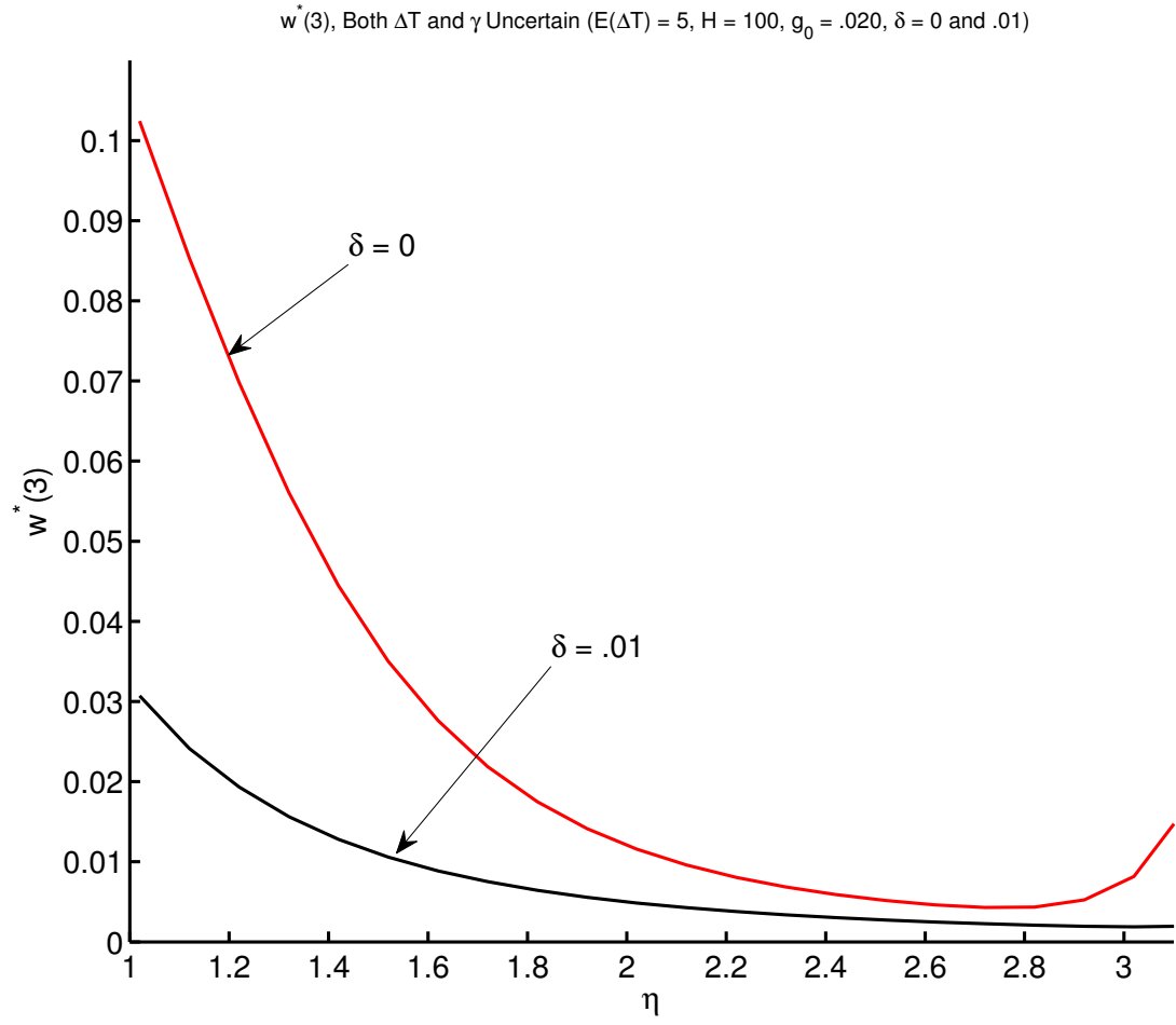
Figure 11: WTP Versus \eta for \tau = 3 . \mathcal{E}(\Delta T_H) = 5^\circ\text{C} , H = 100 , g_0 = .020 , \delta = 0 and .01
