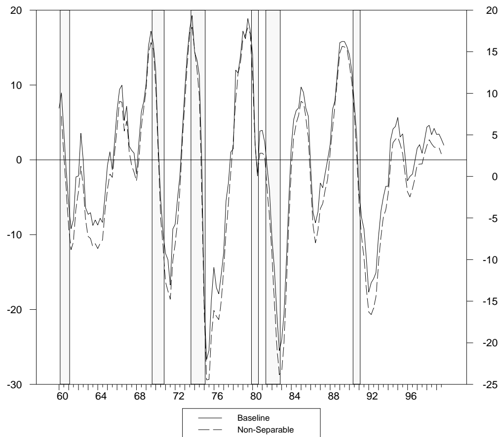
Figure 6. The Gap under Non-Separable Preferences Parameter Values: \sigma=1 , \varphi=5 , \beta=0.99 , b=0.8
