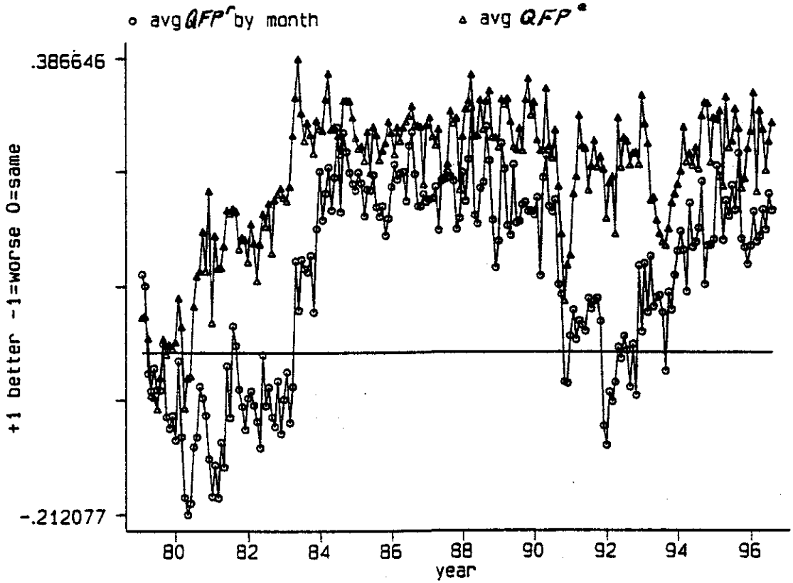
Figure 1: Monthly Averages of QFP r and QFP e
