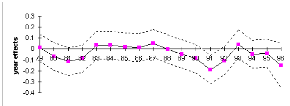
Figure 3: Bias and Time Effects in Forecast Errors Discrete CAB Variables
