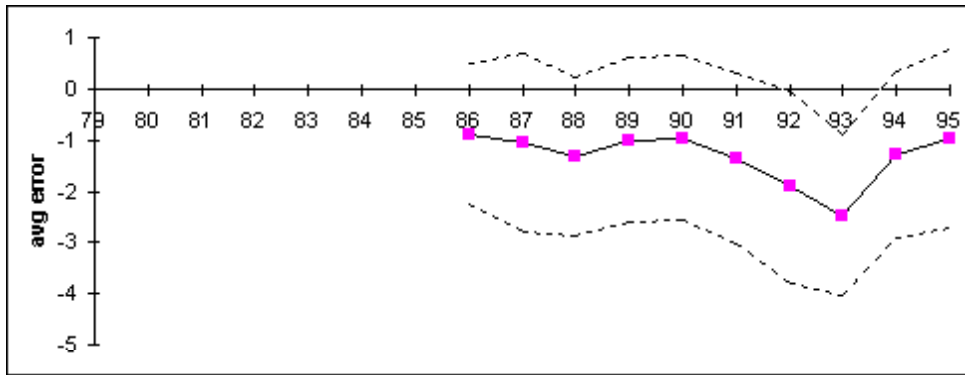
Figure 4: Bias and Time Effects in Forecast Errors Continuous CAB Variables
