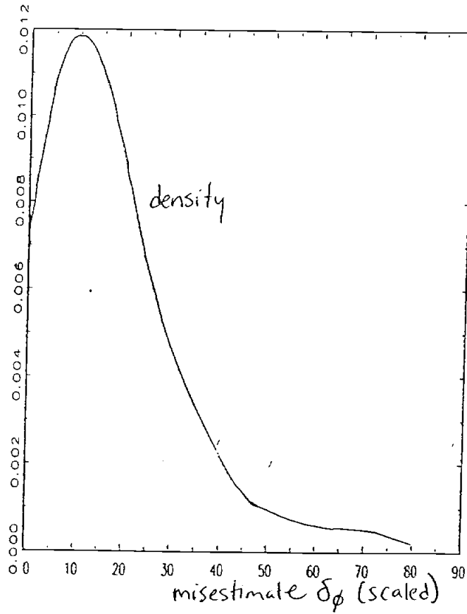
Chart IV: Kernel regression.
