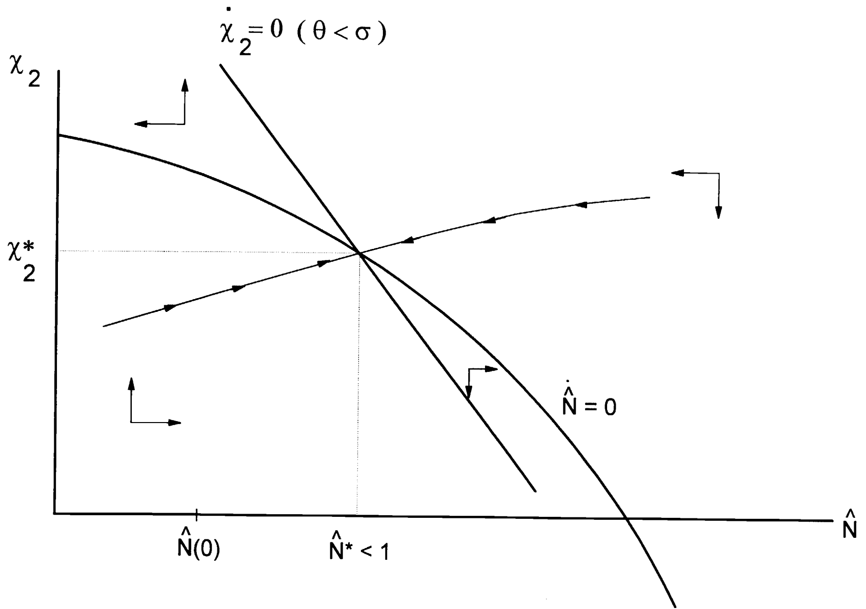
Figure 3. Phase Diagram for country 2 when \theta < \sigma
