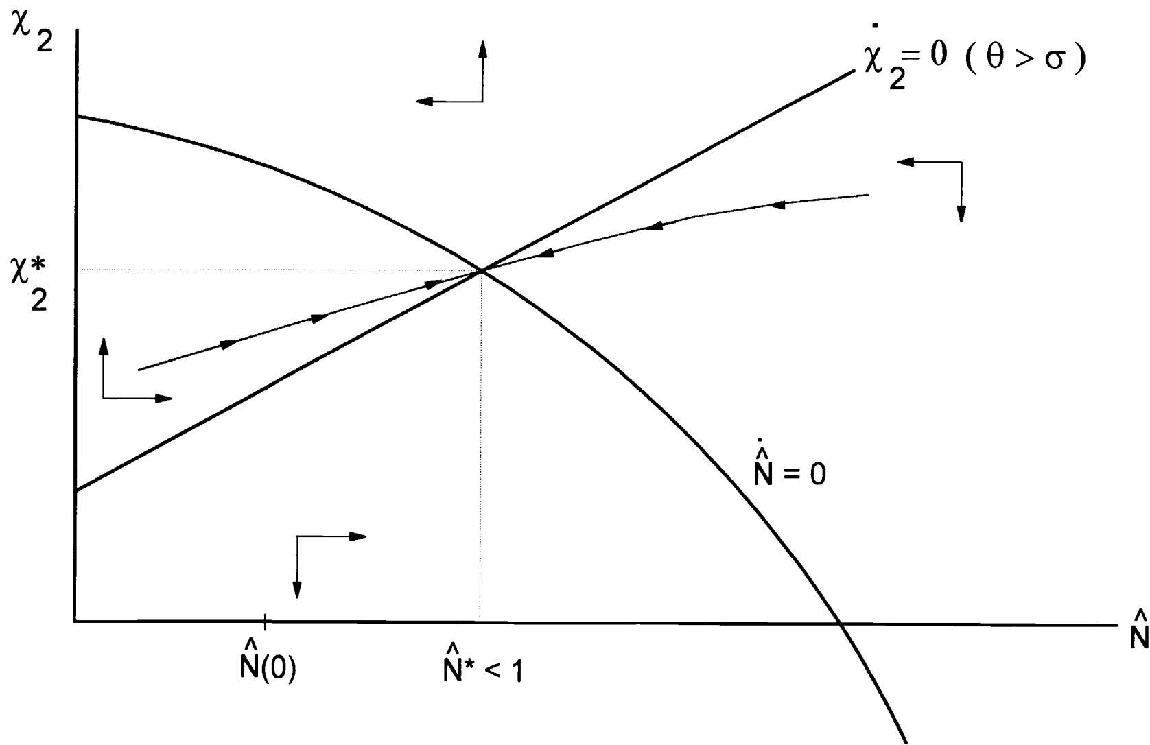
Figure 2. Phase Diagram for Country 2 when \theta > \sigma
