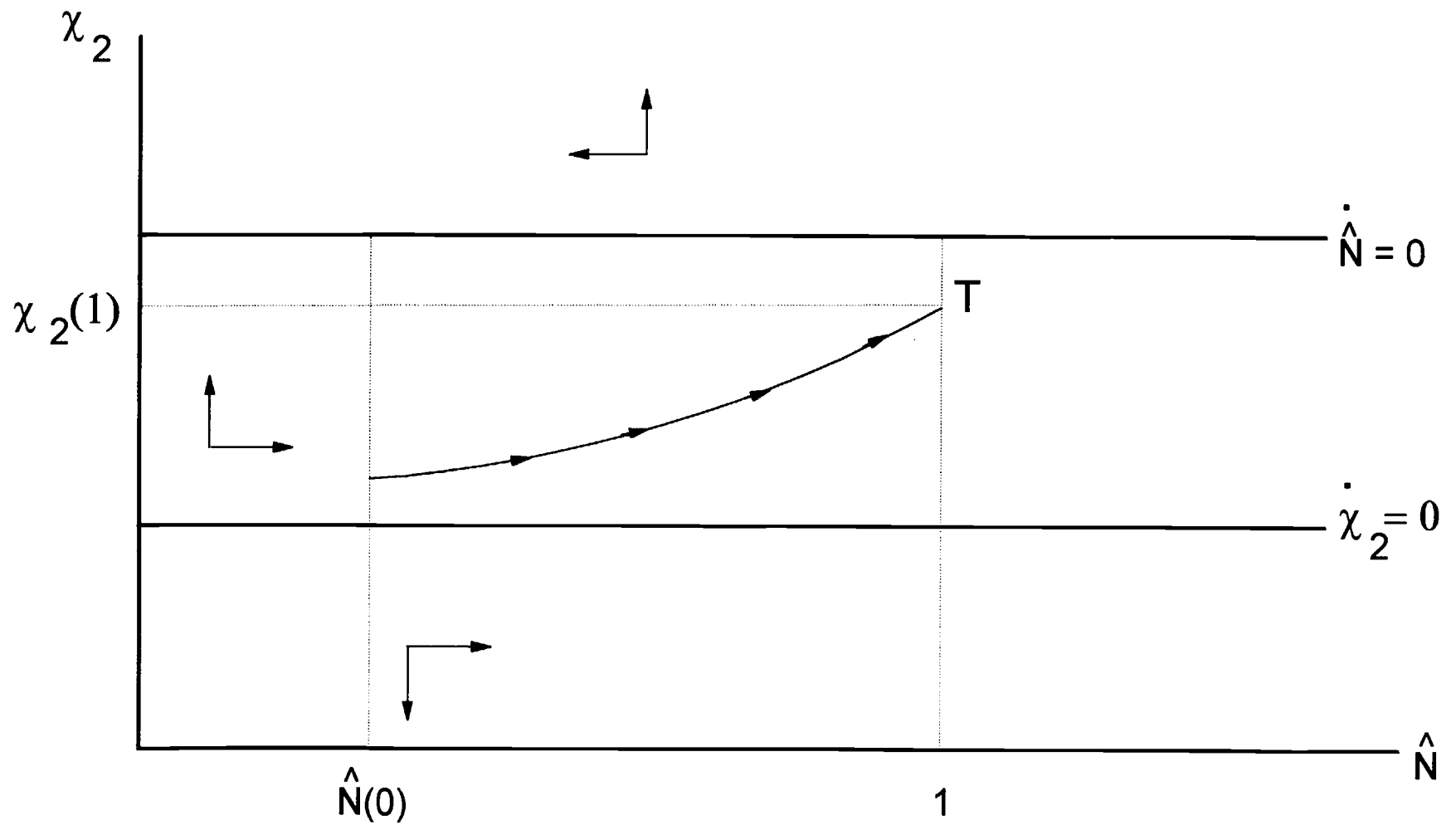
Figure 5. Phase Diagram for Country 2 when v_2 is constant ( \sigma = 0 )
