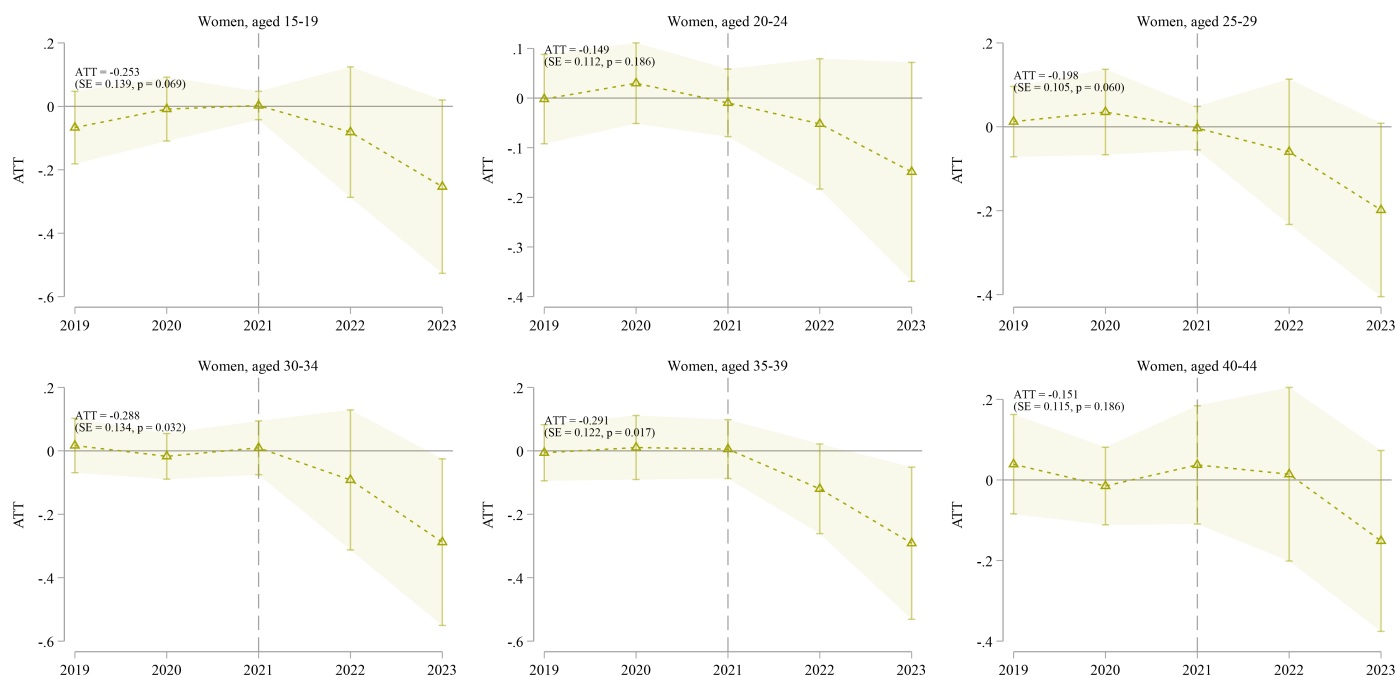
Figure B.2 — SDID event study estimates of the effect of a total abortion ban on female gonorrhea rates, by age group
