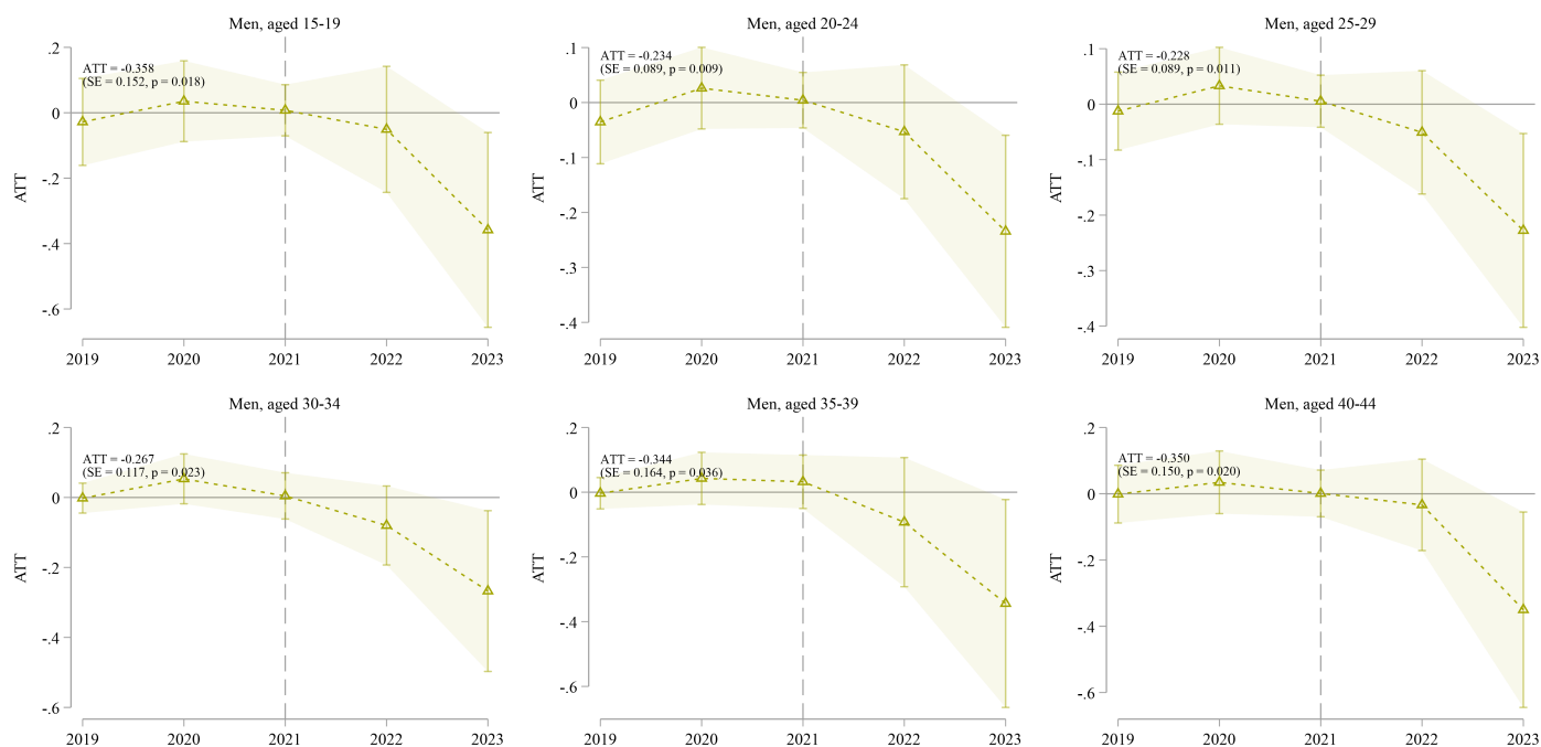
Figure B.1 — SDID event study estimates of the effect of a total abortion ban on male gonorrhea rates, by age group
