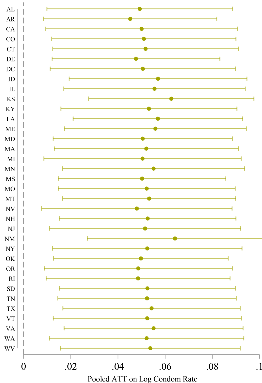
Figure B.22 — Leave-one-out analysis of the effect of a total abortion ban on condom purchases
