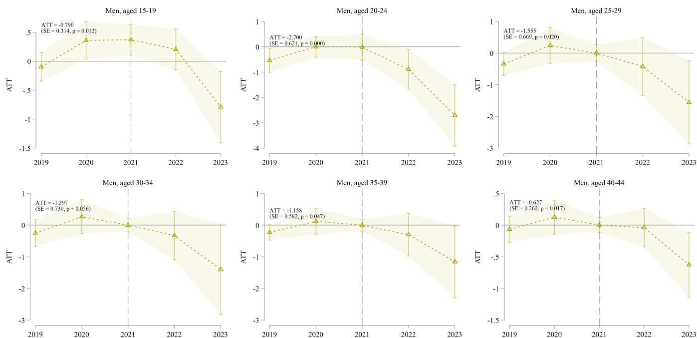
Figure B.3 — SDID event study estimates of the effect of a total abortion ban on male gonorrhea rates, by age group (level)
