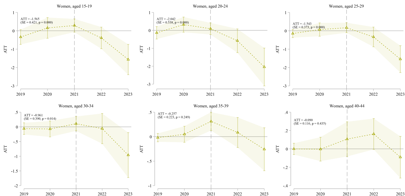
Figure B.4 — SDID event study estimates of the effect of a total abortion ban on female gonorrhea rates, by age group (level)
