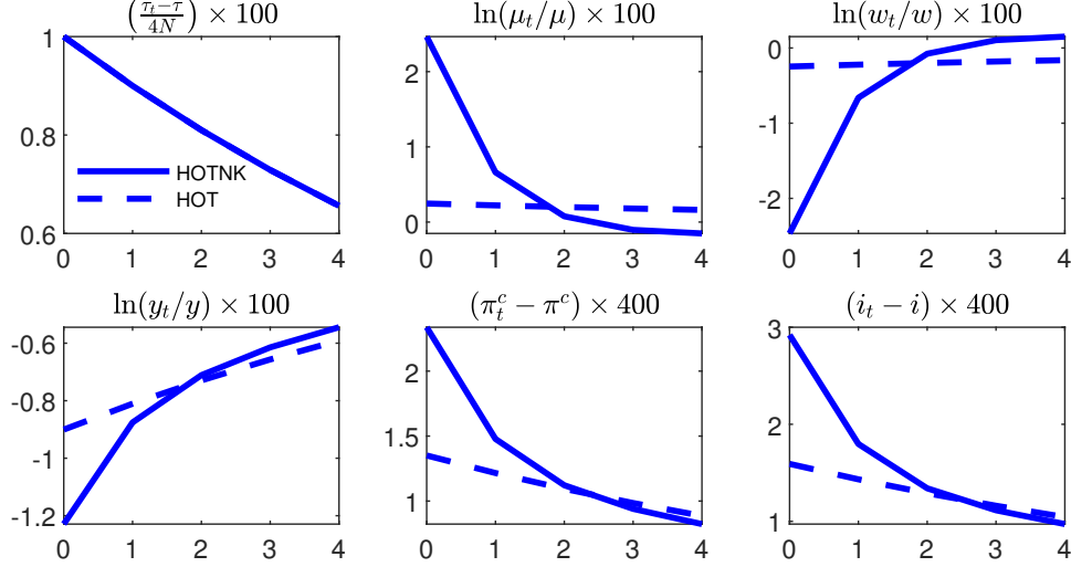
Figure 4: Impulse Response to a Transportation Cost Shock in the HOTNK and HOT Models
