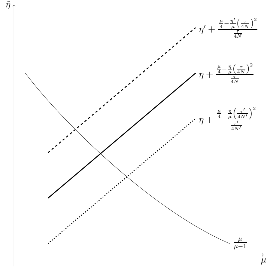
Figure 1: Characterization of the Steady-State Markup
