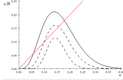
Figure 1: Illustration of fixed point equation (20) for n = 30 (solid top curve), n = 50 (dashed middle curve), and n = 100 (dashed bottom curve).
