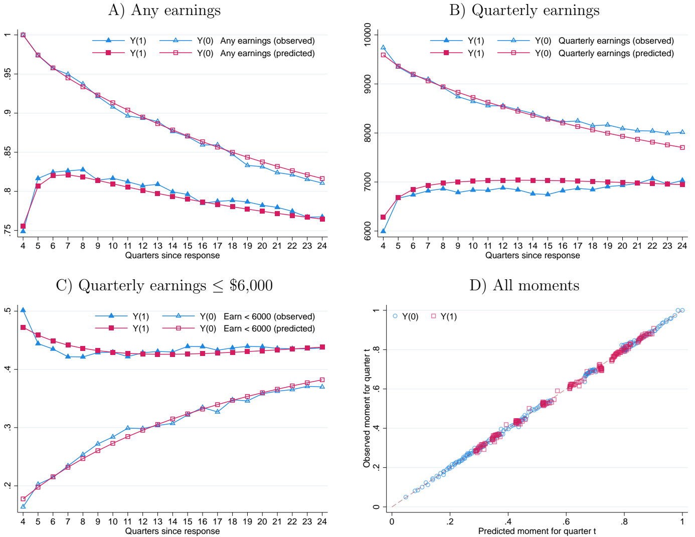
Figure 6: Model fit
