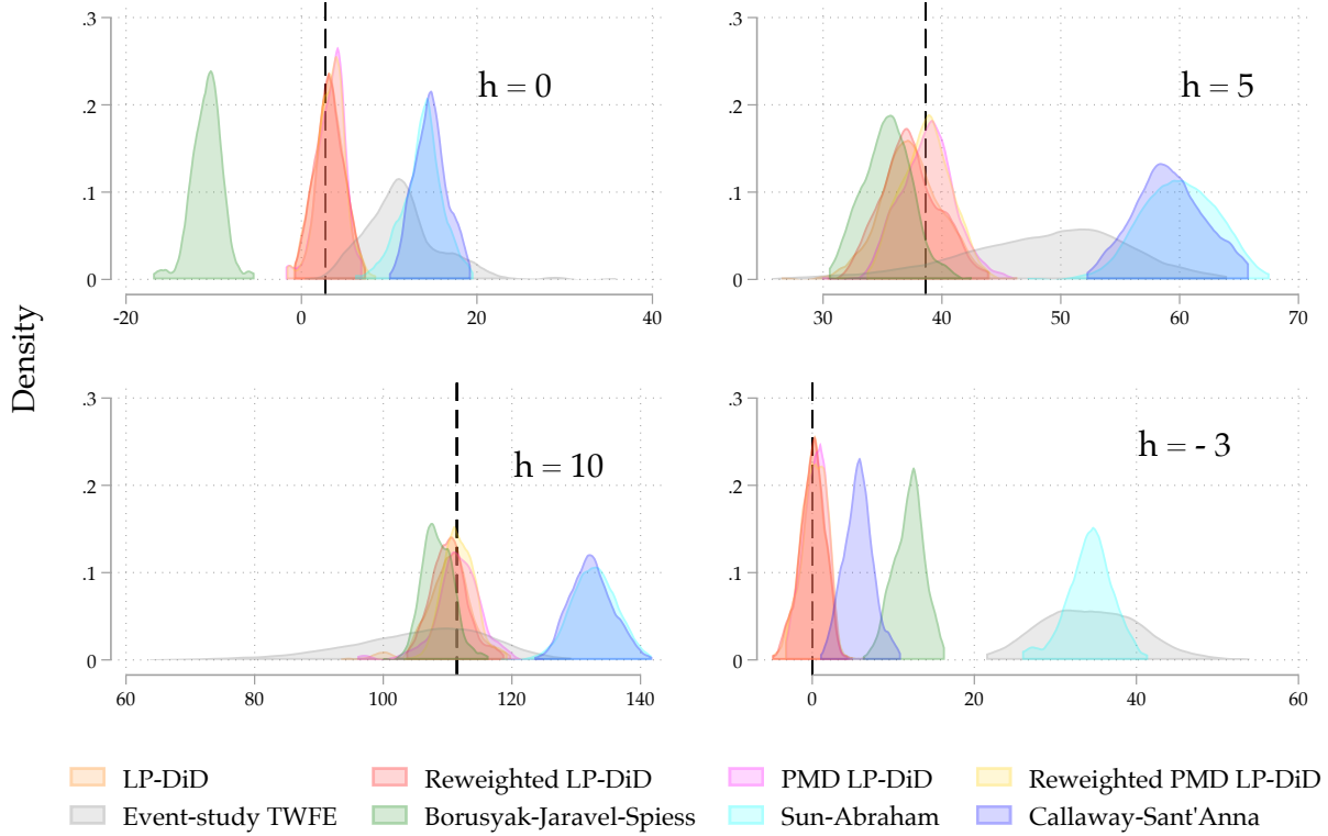
Figure 4: Simulation 2: Endogenous treatment scenario: Distribution of estimates
