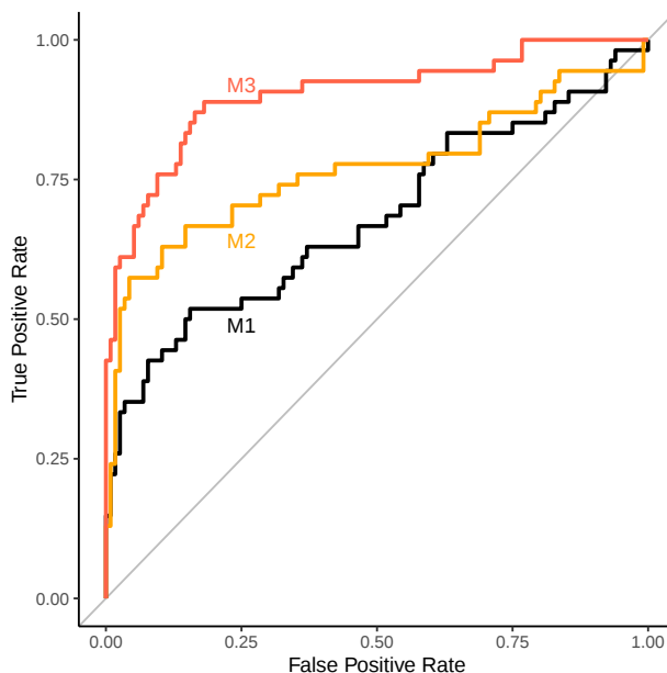
Figure 2: ROC Curves
