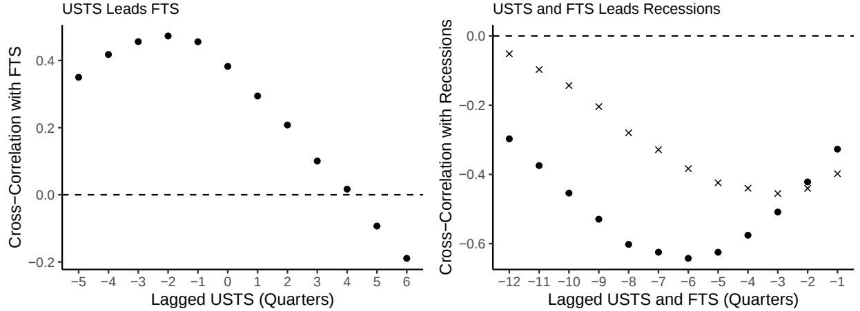
Figure 3: Cross-Correlation Coefficients
