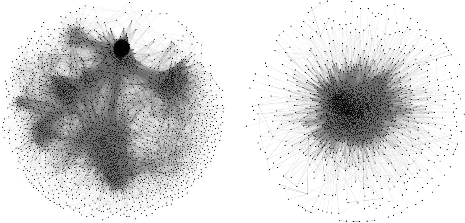
FIGURE 1: NETWORK VISUALIZATION
