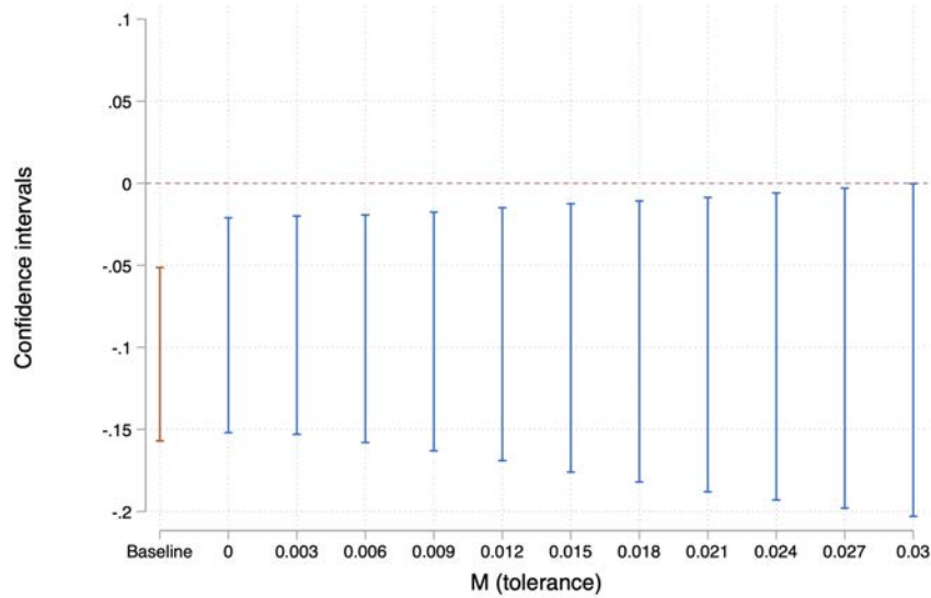
(b) With monotonicity ( \Delta^{SDD}(M) )
