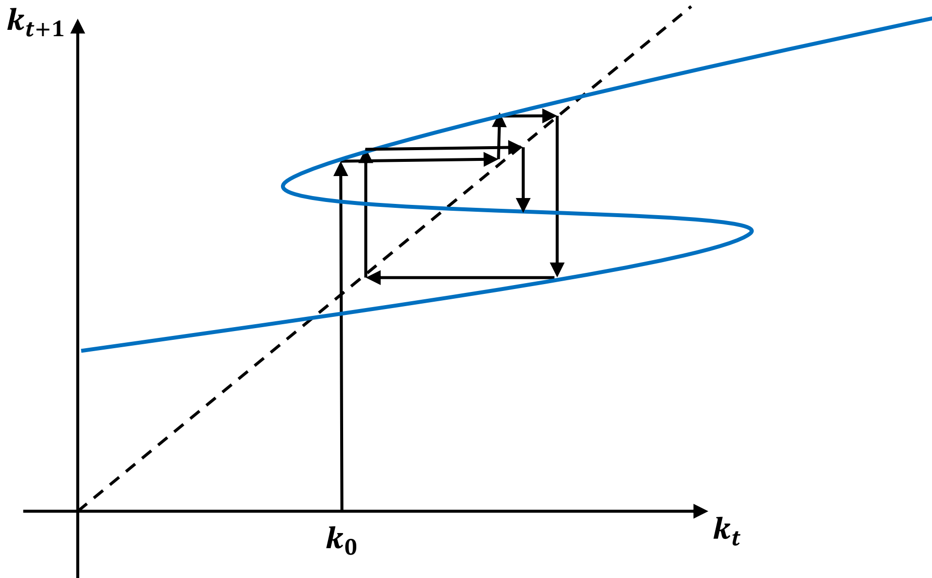
Figure 2-1: A Wobbly Dynamics when P_t = 0
