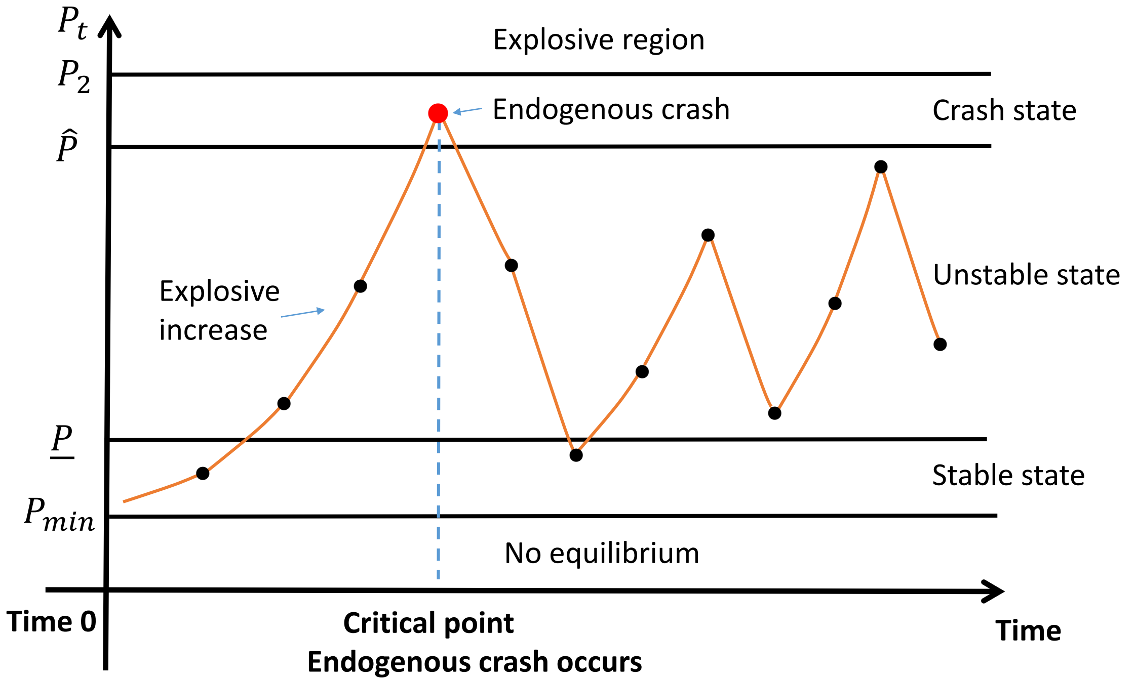
Figure 5: Endogenous Phase Transitions and Endogenous Crash
