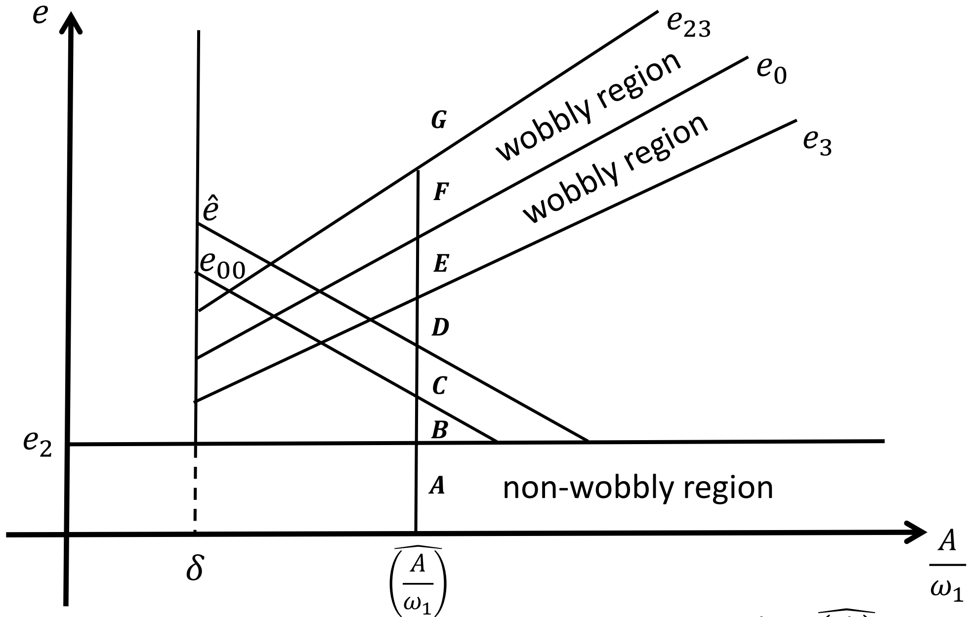
Figure 4-2: Case (b1) e_3 < e < e_{23} and \delta < \frac{a_2}{a_1} and \frac{A}{\omega_1} \geq \overline{\left(\frac{A}{\omega_1}\right)}
