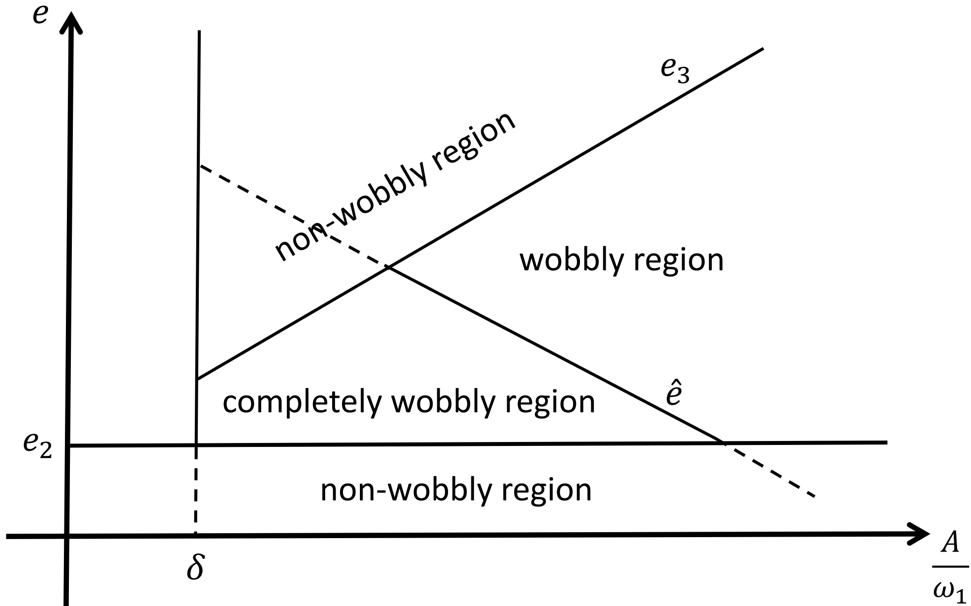
Figure 4-1: Case (a) e_2 < e < e_3 and \frac{A}{\omega_1} > \delta
