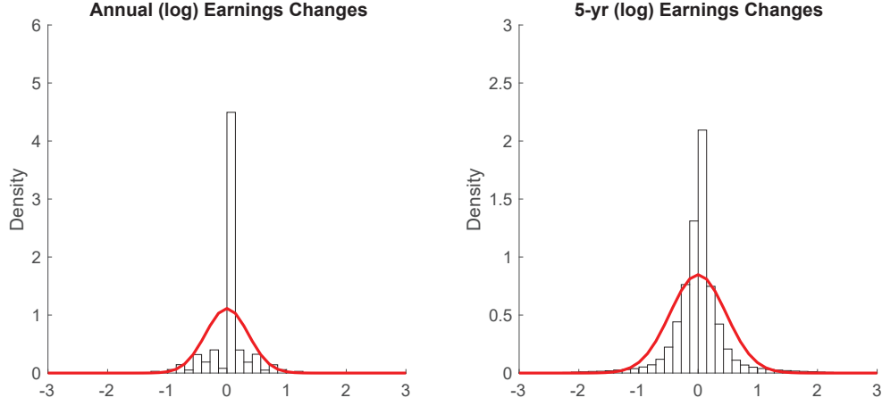
Figure B.1: Distribution of (Log) Income Shocks in the Alternative Calibration
