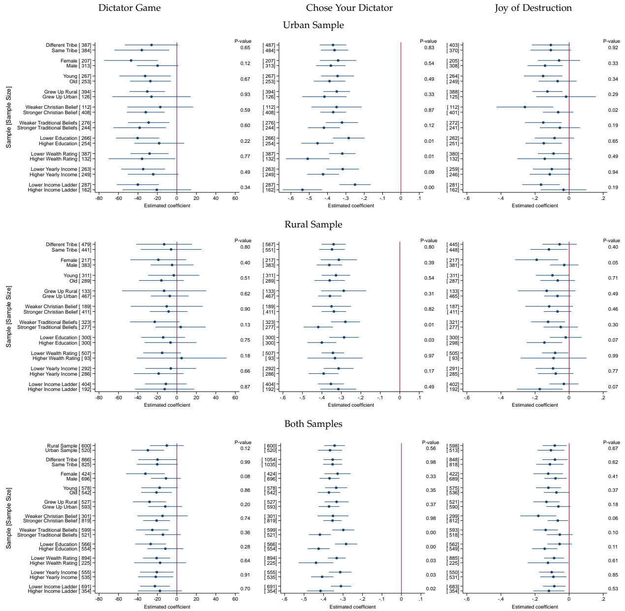
Figure A10: Heterogeneity of Estimates by Player 1 Characteristics and by Game
