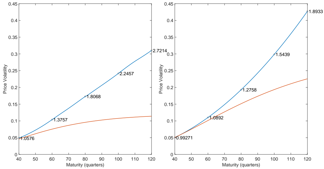
Figure E.5: Giglio-Kelly Variance Ratios: Data and Model
