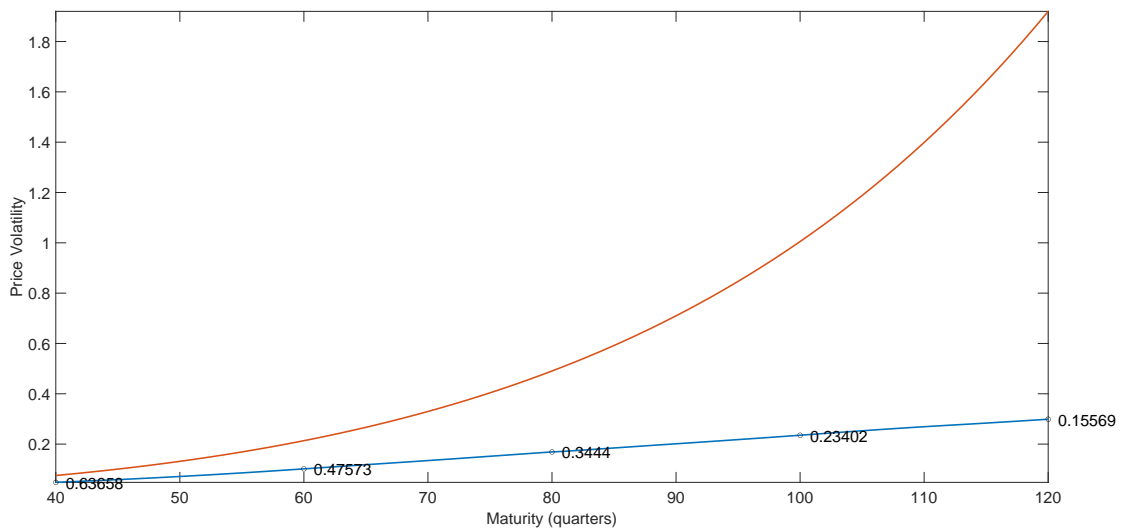
Figure E.6: Giglio-Kelly Variance Ratios for Alternative Basis
