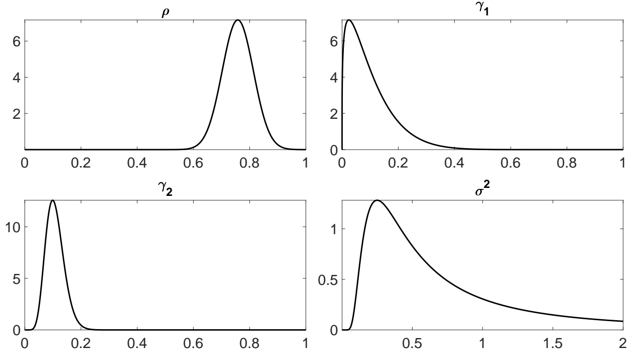
Figure E.1: Marginal Prior Distributions: T-bill Rate Model
