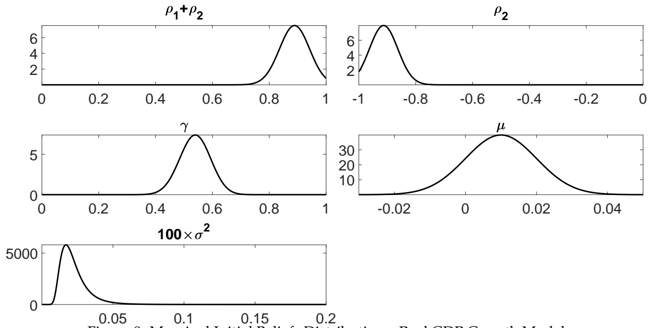
Figure 9: Marginal Initial Beliefs Distributions: Real GDP Growth Model
