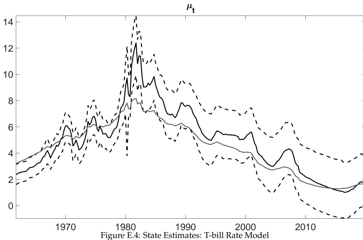
Figure E.4: State Estimates: T-bill Rate Model Note: Each panel corresponds to one of the two UC hidden state variables: \mu_t and x_t respectively. The black solid line is the posterior mean of the real-time filtering distributions, the dotted black lines are the 5th and 95th percentiles of the posterior real-time filtering distributions, and the solid gray line is the posterior mean of the ex-post smoothing distributions for the corresponding parameter.
