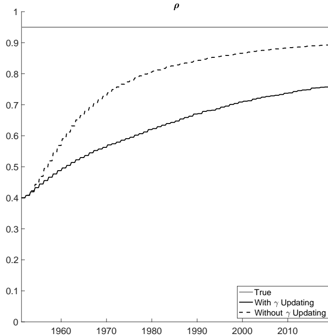
Figure 14: Learning about Persistence with Different Values for \gamma
