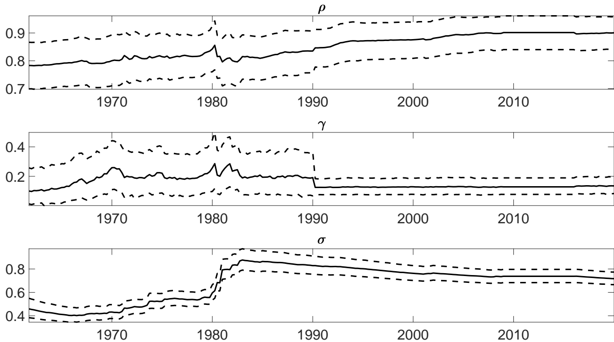
Figure E.3: Parameter Estimates: T-bill Rate Model
