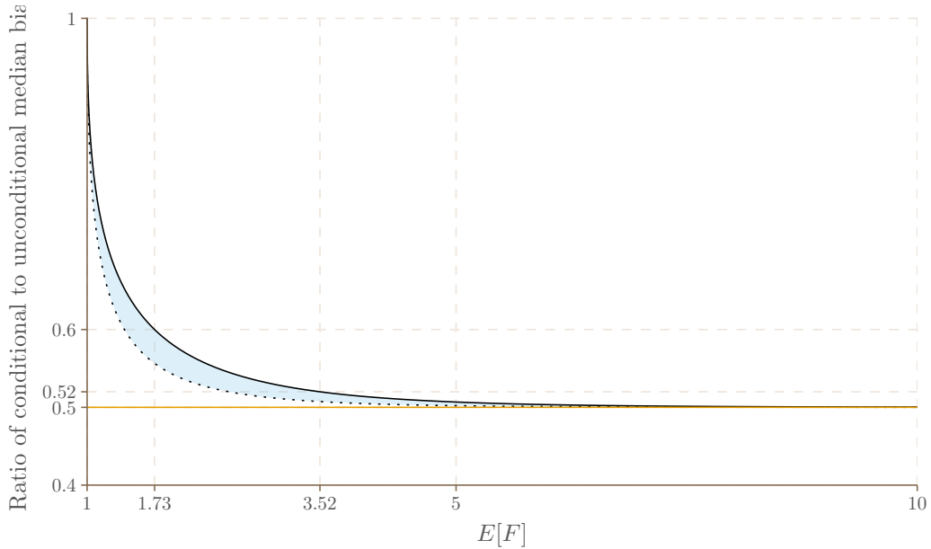
Figure 3: Median bias of \hat{\beta}_{IV} conditional on t_1 > 0 relative to unconditional median bias. Solid line denotes the ratio when \rho = 1 , dotted line denotes the limit as \rho \rightarrow 0 , and blue shaded area denotes the range of possible values over the possible values of \rho . Solid orange line marks a reference line at 0.5. See Appendix A.6 for computational details.
