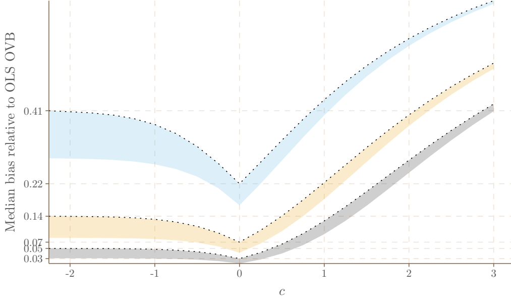
Figure 2: Relative median bias of \hat{\beta}_{IV} conditional on t_1 > c , \text{median}(\hat{\beta}_{IV} - \beta \mid t_1 > c) / |\beta_{WOLS} - \beta| as a function of cutoff c for selected values of E[F] . Shaded areas delineate the range of variation in the relative bias over possible values of \rho . Blue: E[F] = 2 , orange E[F] = 3.5 , gray: E[F] = 5 . Dotted lines denote the limit of the relative bias as \rho \rightarrow 0 . See Appendix A.6 for computational details.
