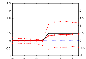
Appendix Figure A2: Synthetic control estimators across DGPs. The true treatment effect is depicted in solid black. For each value of k indicated on the x-axis, the series correspond to the 2.5th (dotted, marked by x's), 50th (solid, marked by +'s), and 97.5th (dotted, marked by x's) percentiles across 1000 simulations for each \hat{\delta}_k . The right axis depicts the estimated treatment effect relative to the synthetic control. On the left axis, estimates are normalized such that the median treatment effect is zero the period before the event. The donor pool for unit i in cohort t^*(i) consists of all units j with t^*(j) > t^*(i) + 5 and all units j that never adopt the policy, and weights are chosen to fit the path of the outcome variable in all periods prior to t^*(i) . The first row ("Two-way fixed effects") implements a two-way fixed effects estimator. The second row ("Synthetic control (Simplex)") estimates \hat{\delta}_k using the synth package (Abadie et al. 2020), restricting the weights on the donor units to the simplex. The third row ("Synthetic control (Unconstrained)") estimates \hat{\delta}_k using the augsynth package (Ben-Michael et al. 2020), allowing donor weights outside the simplex but imposing an \ell_2 -penalty of 0.001.
