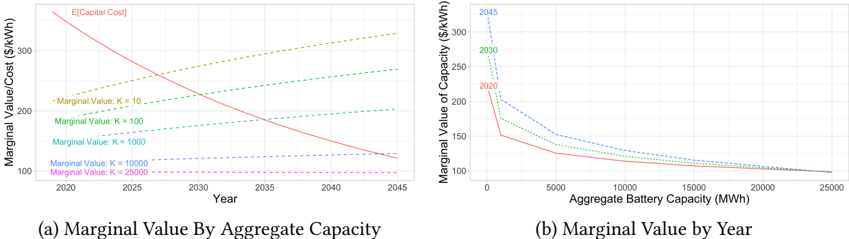
Figure 7: Marginal Value and Cost of Battery Investment Over Time
