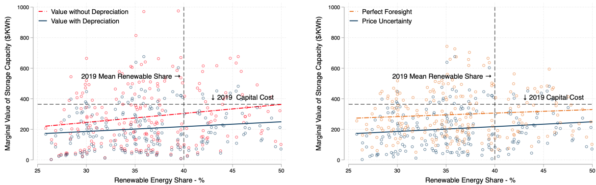
(a) Battery Depreciation and Battery Value
