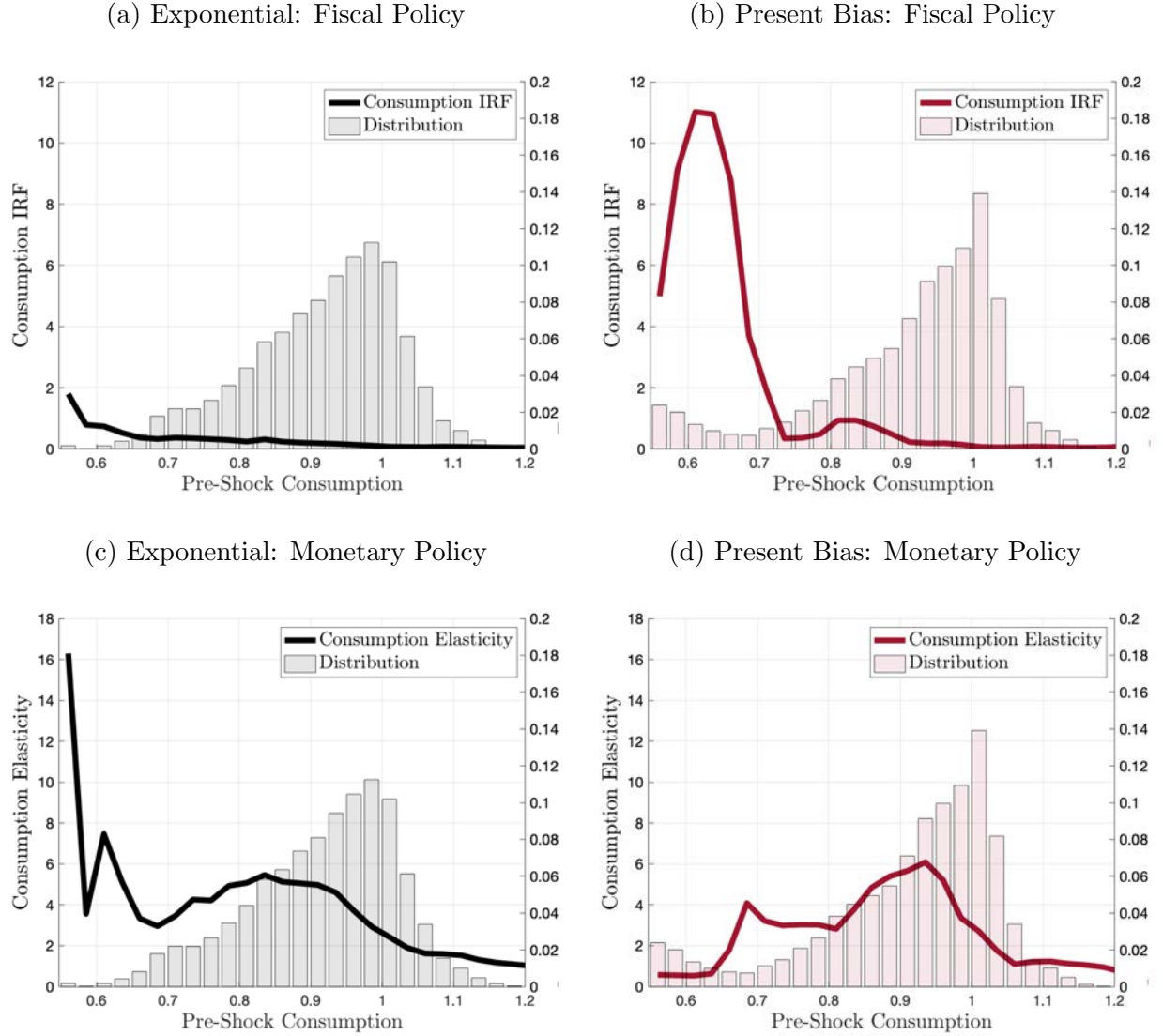
Figure 8: Heterogeneity Analysis.
