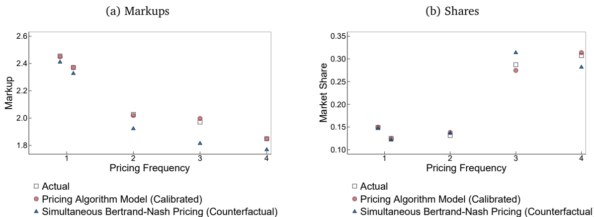
Figure 14: Calibration Fit for Markups and Shares
