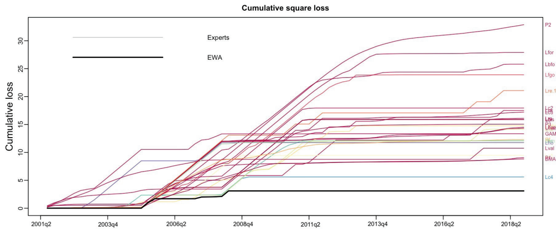
Figure 5: France: Experts. Quasi-real time. Cumulative Loss. EWA aggregation.
