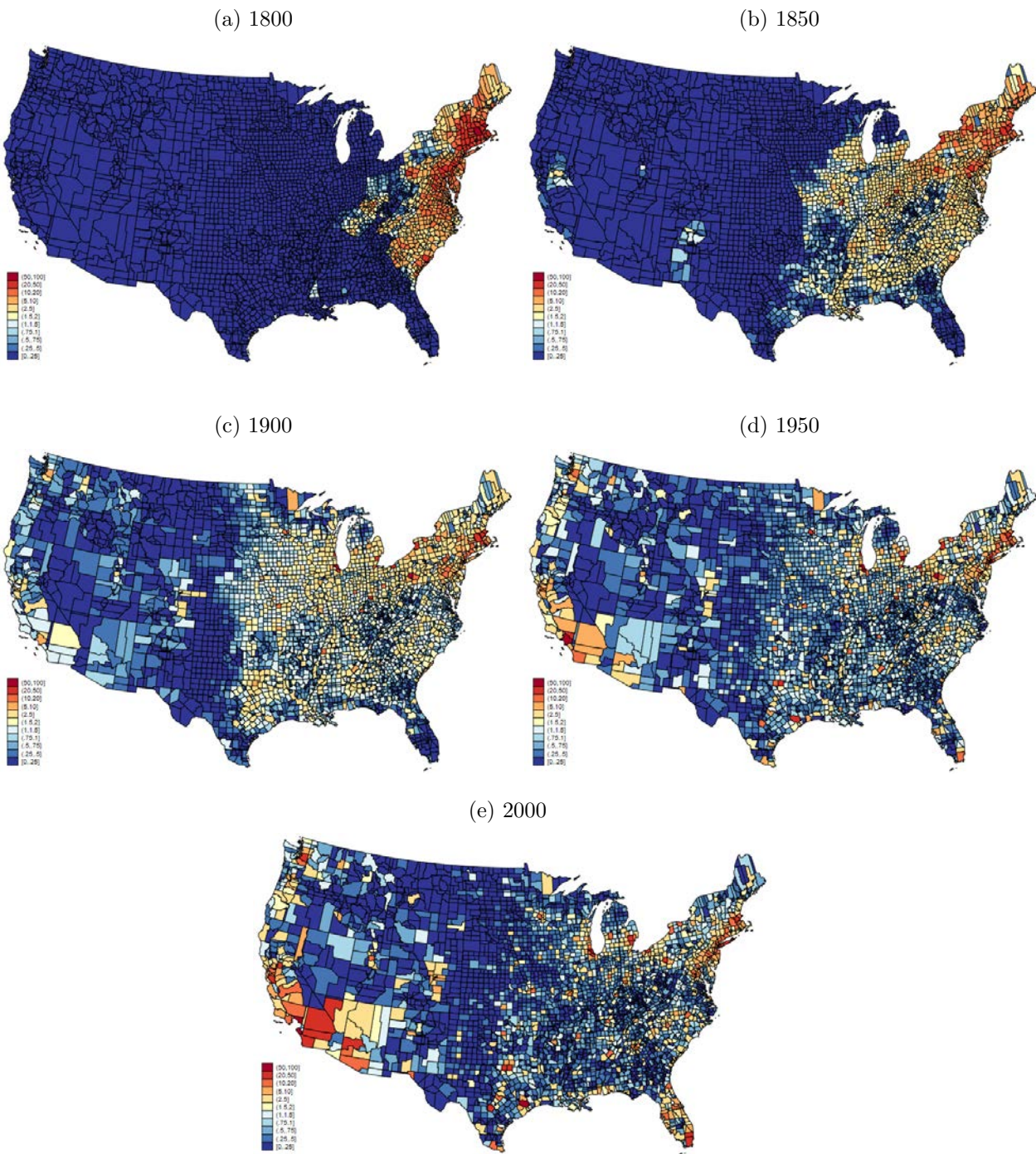
Figure C.1: Spatial distributions of population over time
