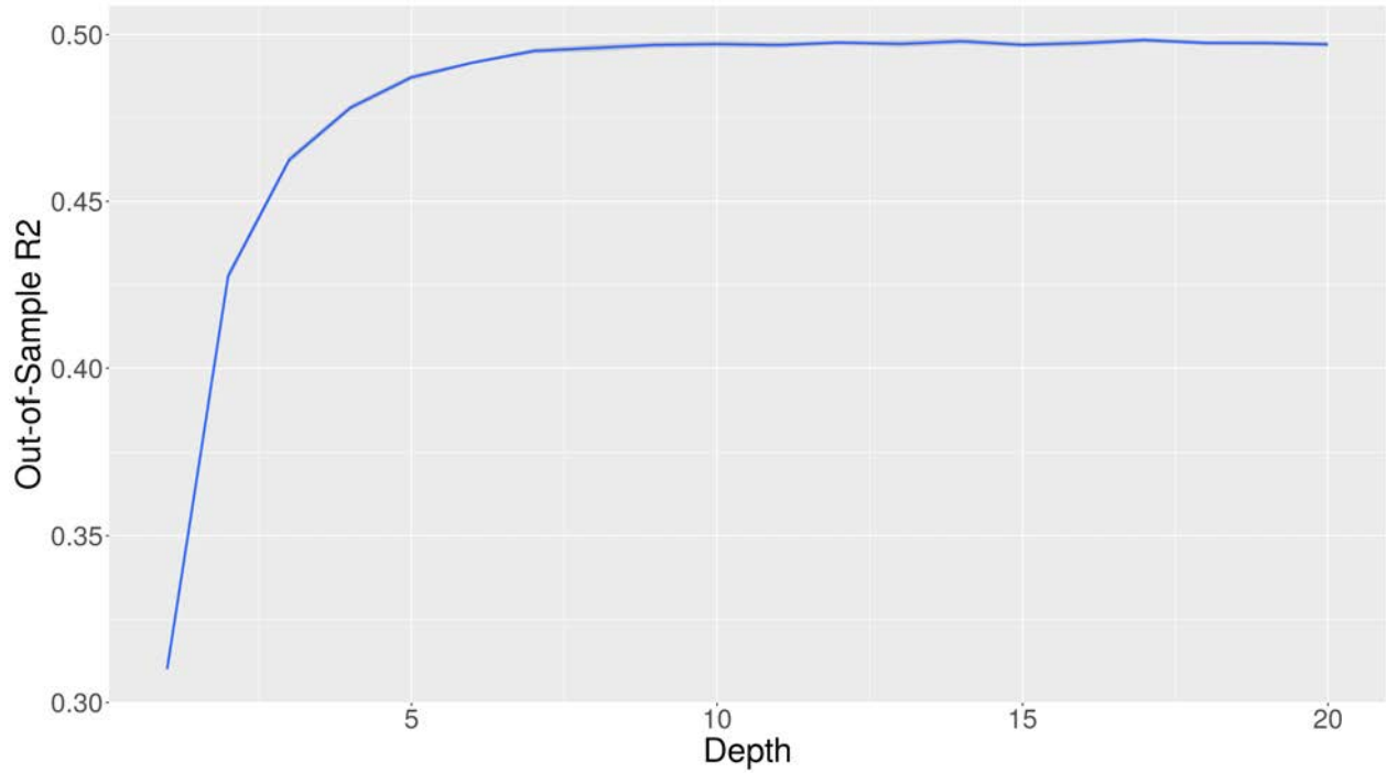
Figure 8: Cross-validation results of the maximum depth of each tree in the one-quarter-ahead forecast
