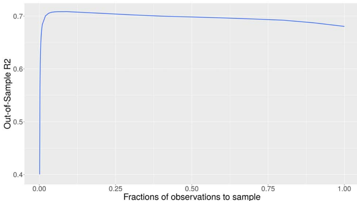
Figure 11: Cross-validation results of the fraction of the sample that is taken in each split in the one-year-ahead forecast
