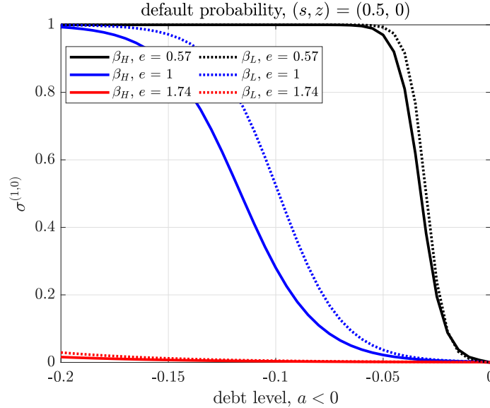
Figure 2: Default Probability by Earnings and Type
