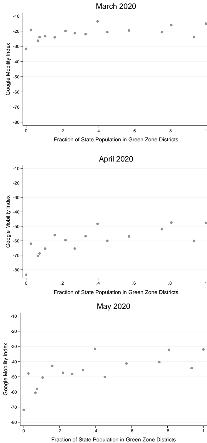
Figure A.4: Correlations Between Fraction of State Population in Green Lockdown Districts & Google Mobility Index
