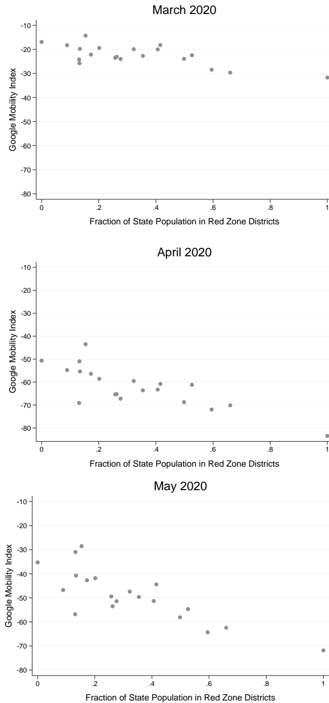
Figure A.2: Correlations Between Fraction of State Population in Red Lockdown Districts & Google Mobility Index
