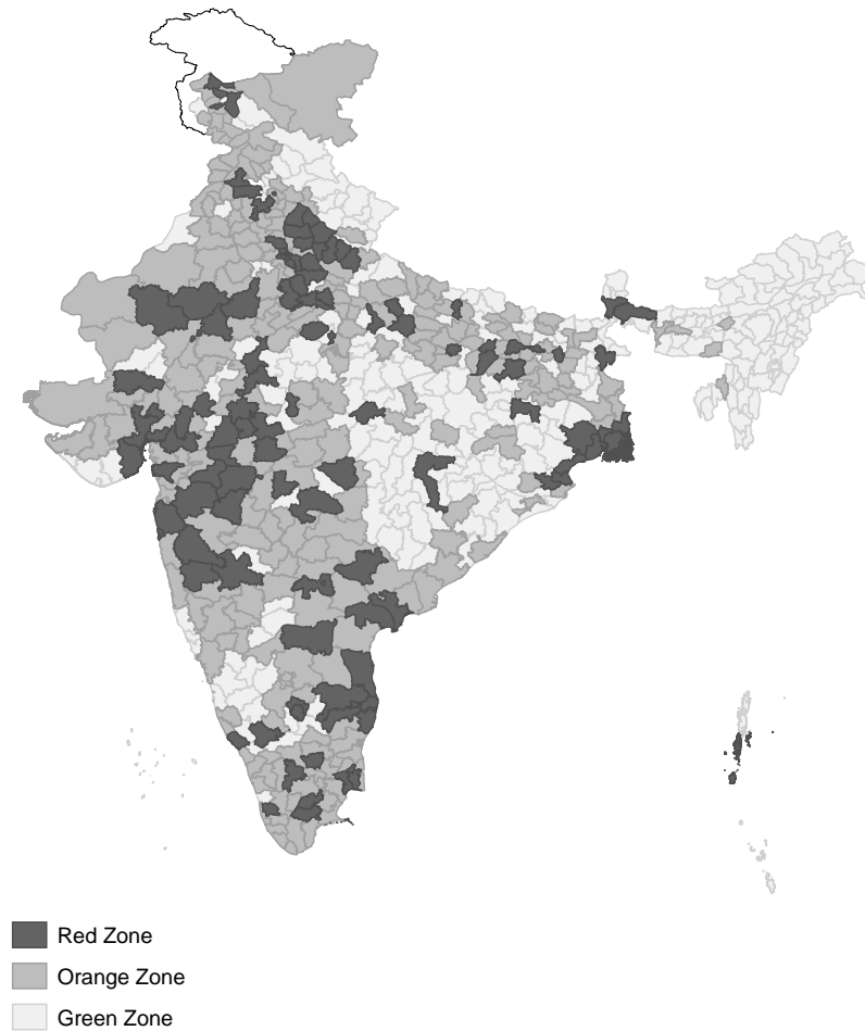
Figure A.1: Spatial Distribution of Red, Orange & Green Lockdown Districts
