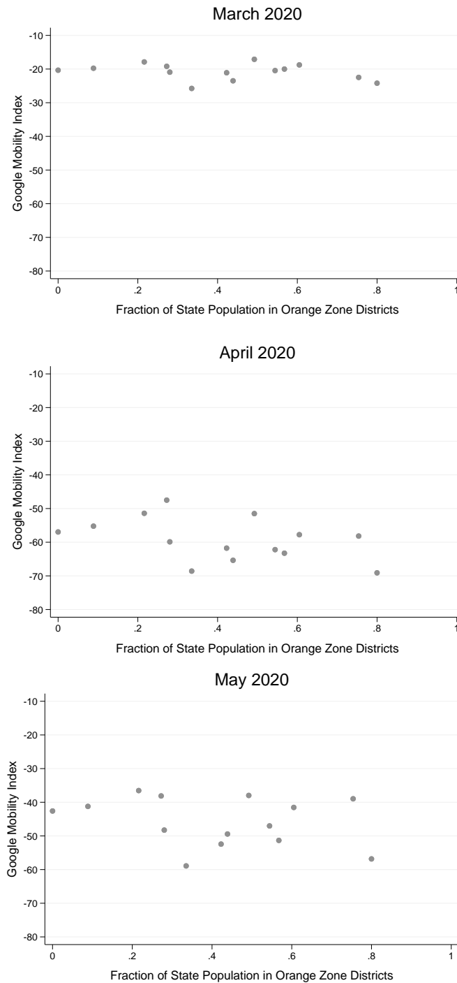
Figure A.3: Correlations Between Fraction of State Population in Orange Lockdown Districts & Google Mobility Index
