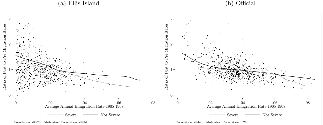
Figure 4: \beta -convergence in emigration rates
