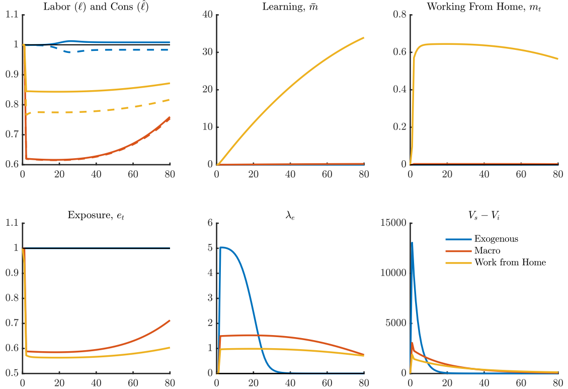
Figure 6: Planner Solution: Aggregates with Smaller Infection Shock
