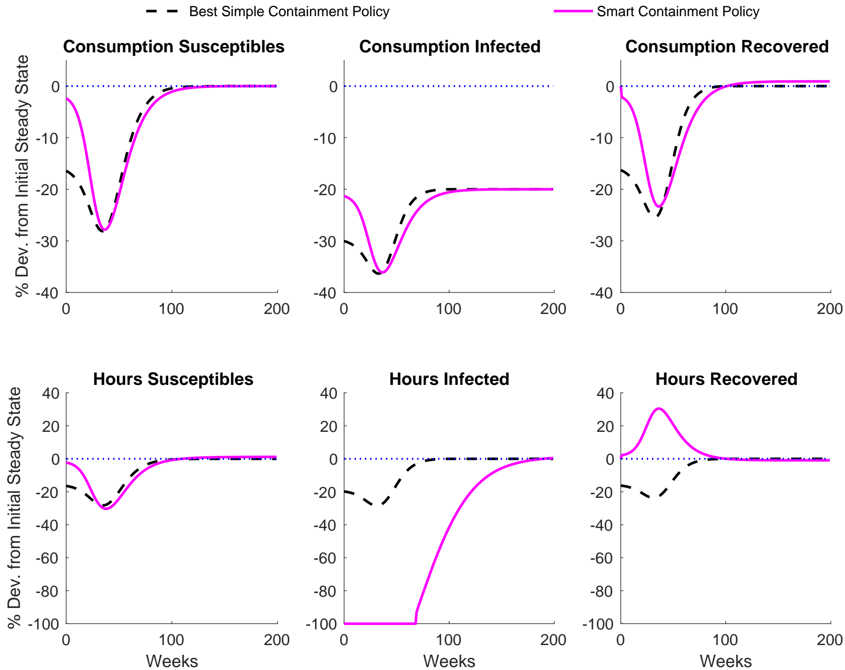
Figure 11: Best Simple vs. Smart Containment in Benchmark SIR-Macro Model
