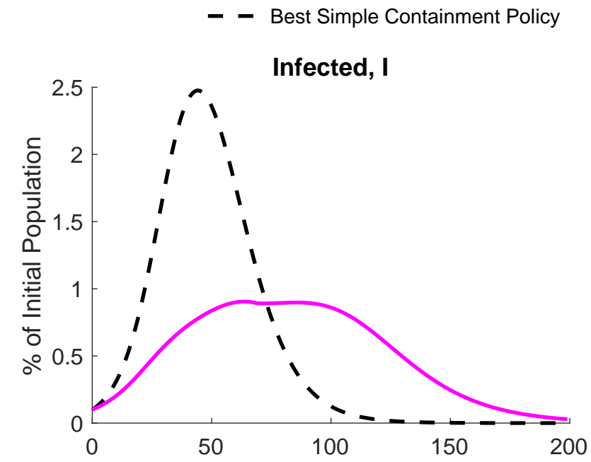
Figure 10: Best Simple vs. Smart Containment in Benchmark SIR-Macro Model
