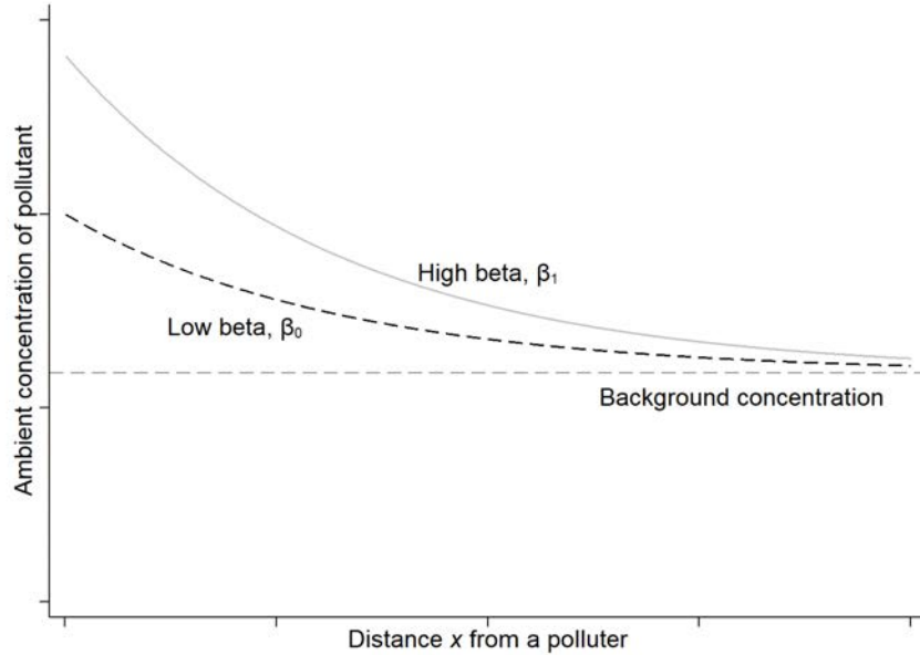
Figure 1: Exponential Decay of Pollution
