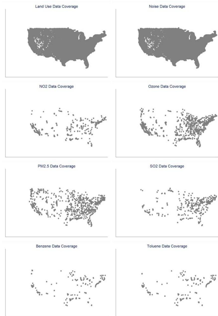
Figure A3: Data Coverage
