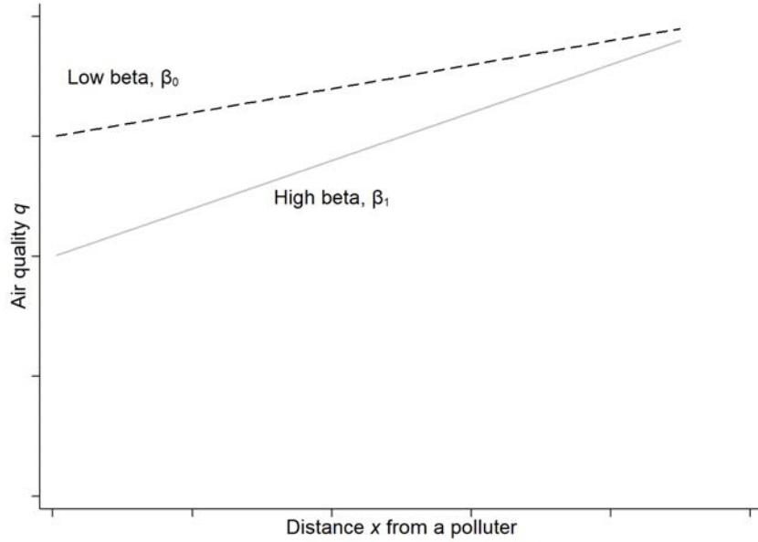
Figure 2: Environmental Quality Increases with Distance
