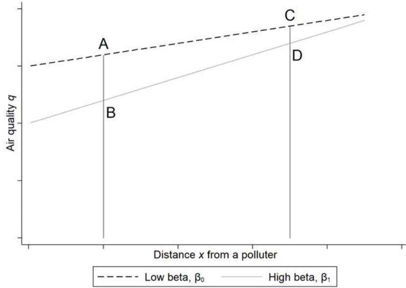
Figure 3: Incorrect Information Regarding Air Quality
