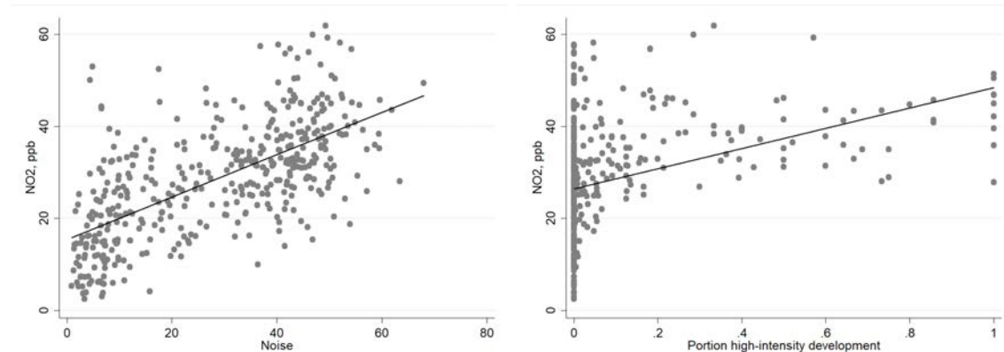
Figure 5: Noise and Land Use Are Correlated with Pollution Exposure
