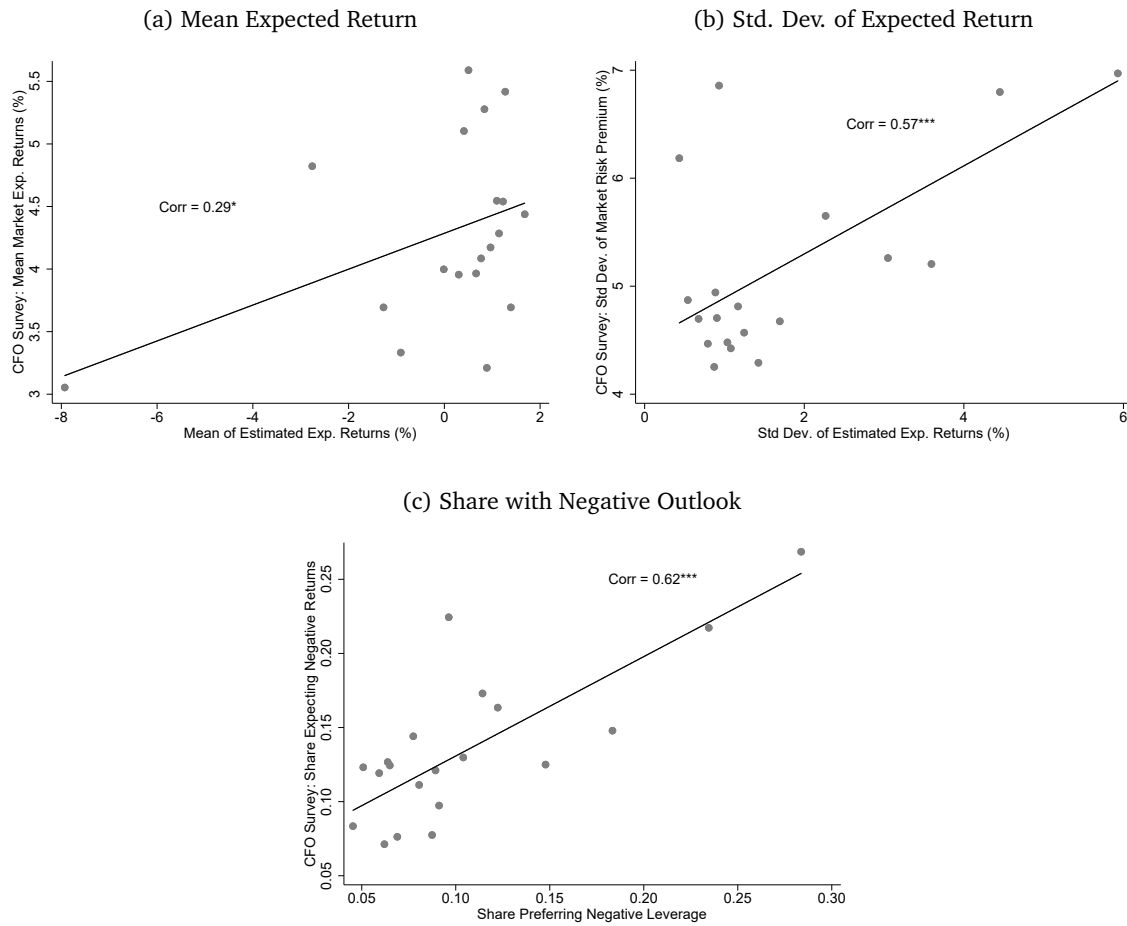
Figure A11: Comparison with Duke CFO Global Business Outlook Survey
