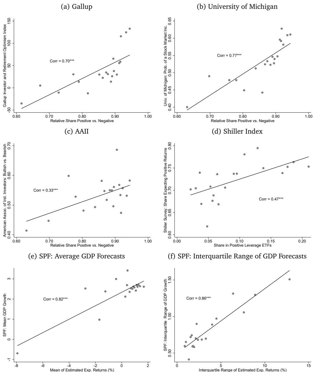
Figure A12: Comparison with Surveys
