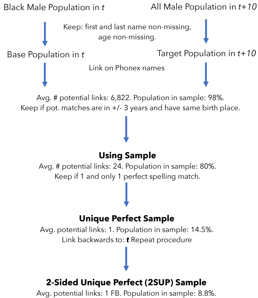
Figure A.4: 2SUP Linking Algorithm
