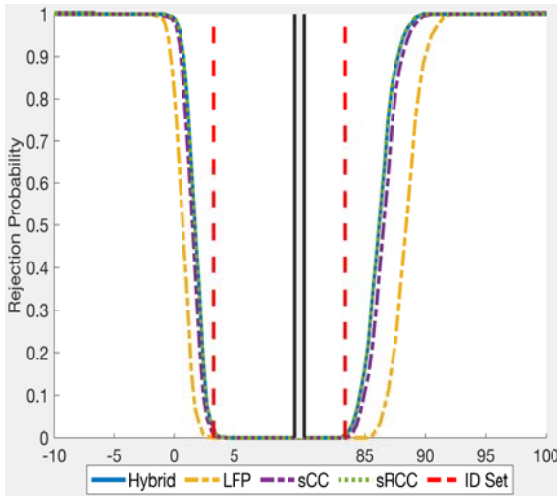
(e) 10 Parameters, 38 Moments
