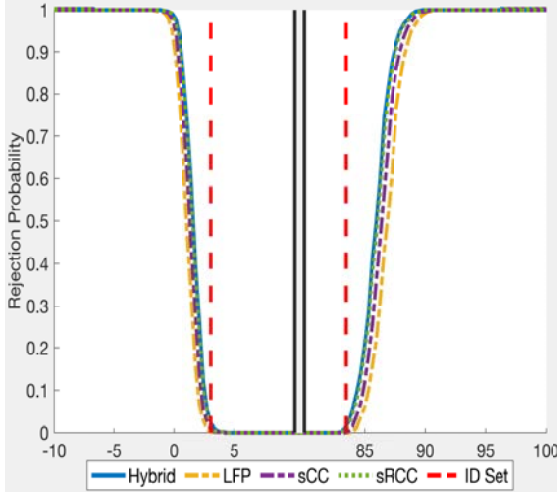
(c) 4 Parameters, 14 Moments
