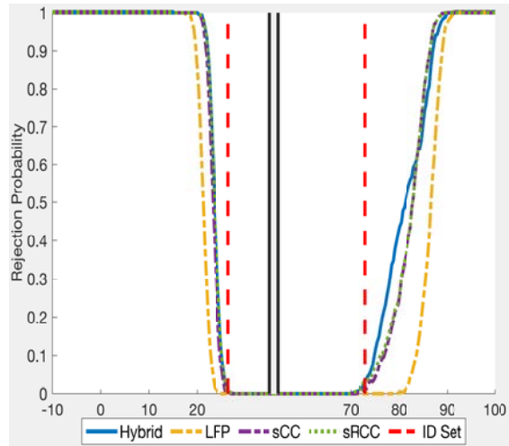
(f) 10 Parameters, 110 Moments
