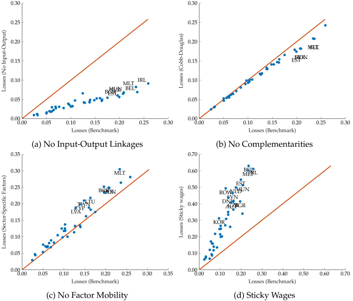
Figure 5: Log reduction in welfare by country in response to a 60% increase in iceberg trade costs. The x -axis is the reduction implied by the benchmark model and the y -axis is the reduction under alternative assumptions. Countries with the largest deviation from the 45-degree line are labelled. If a country is above the 45-degree line, then the response of welfare is stronger relative to benchmark. Luxembourg has been removed for readability since it is an outlier.
