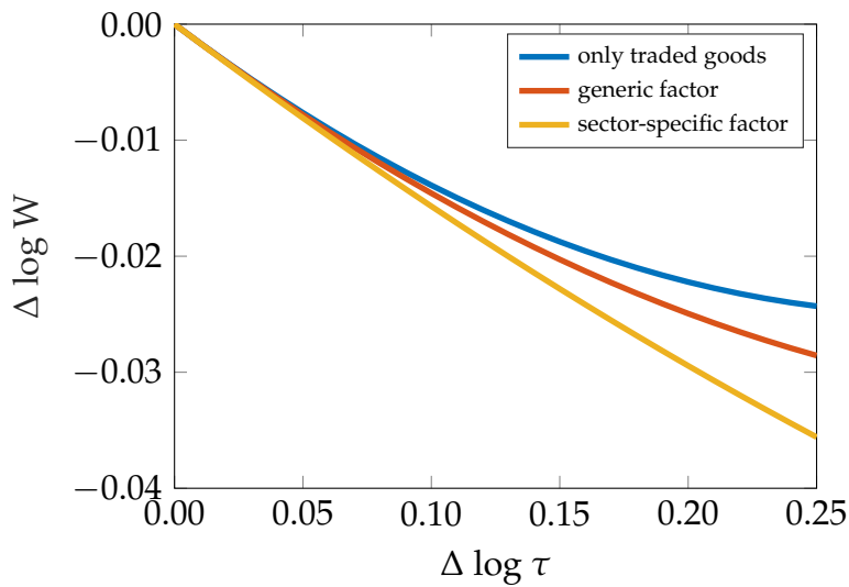
Figure 2: The change in welfare implied by (13) for the case with no non-traded goods ( \sigma = \theta ), generic factor only ( \alpha = 1 ), and sector-specific factors only ( \alpha = 0 ). In all cases, the import share of consumption is kept constant at \lambda_T^{W_c} = 1/6 , so the different specifications are all first-order equivalent. The elasticity of substitution across traded goods is \theta = 5 and across sectors is \sigma = 0.1 .
