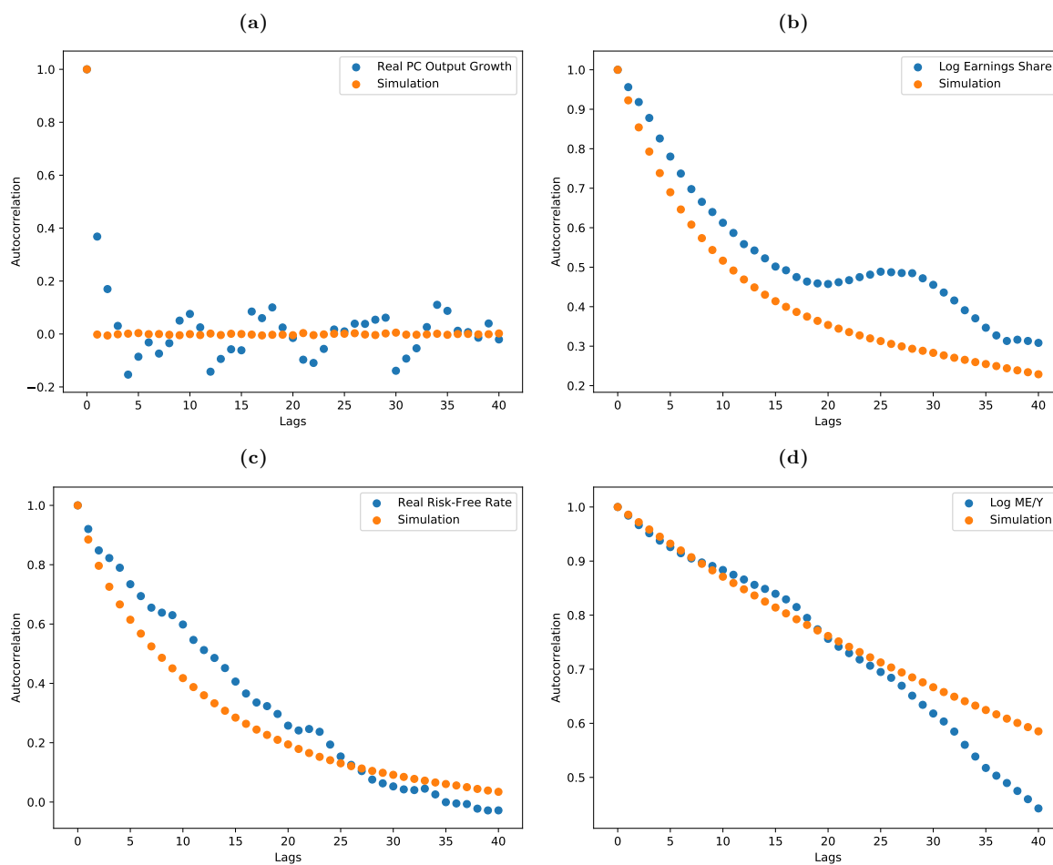
Figure 11: Observable Autocorrelations
