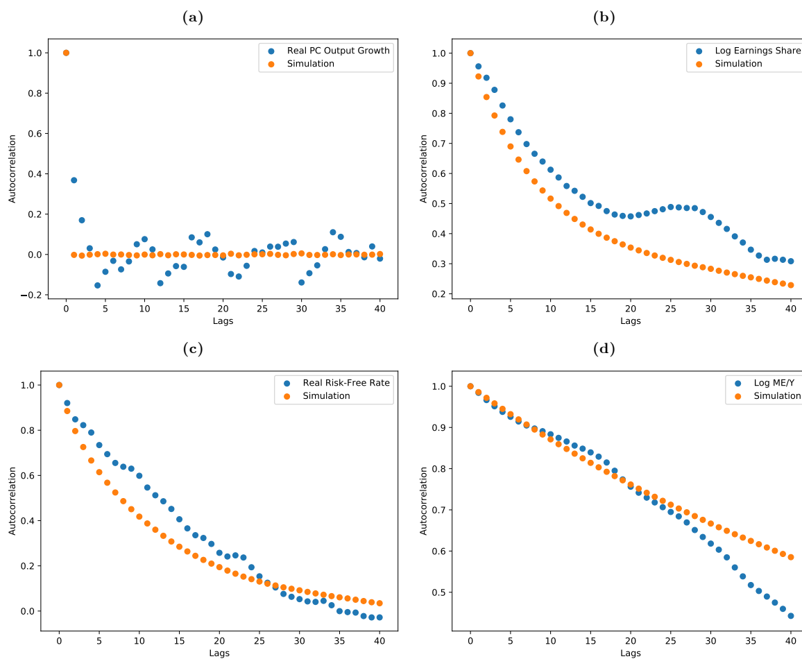
Figure 10: Observable Autocorrelations
