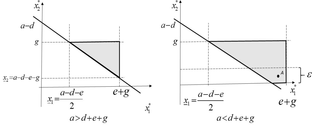
Figure 4: The existence of a Grand Coalition Equilibrium
