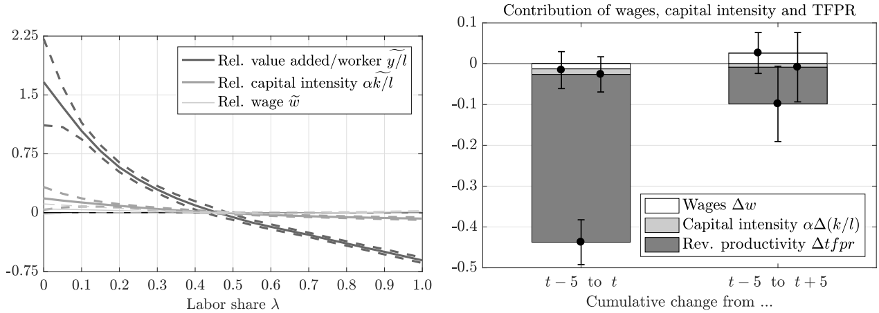
Figure 11: Labor productivity dominates cross-sectional differences and time-series dynamics of labor shares of HP establishments.
