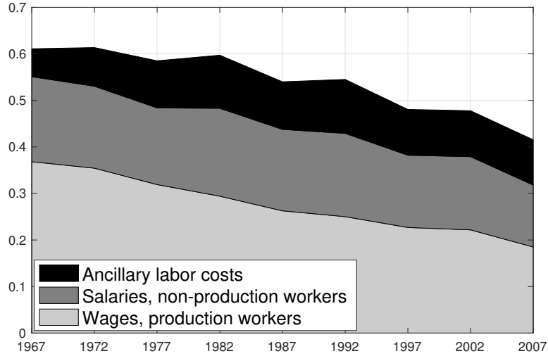
Figure 16: Dynamics of labor share components
