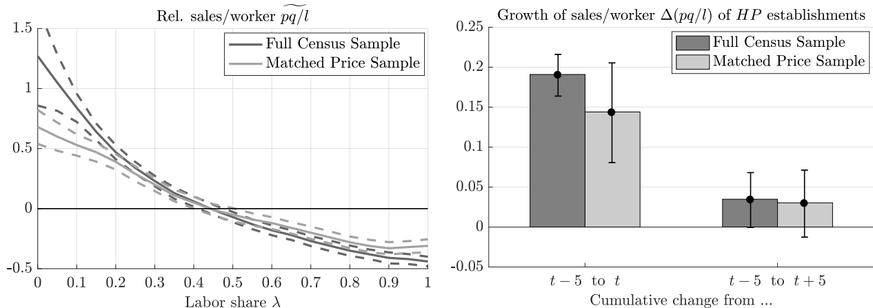
Figure A.1: Relative sales per worker in the Full Census Sample vs. the Matched Price Sample
