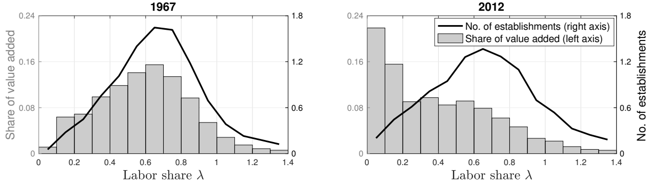
Figure 1: The changing distributions of labor shares and value added
