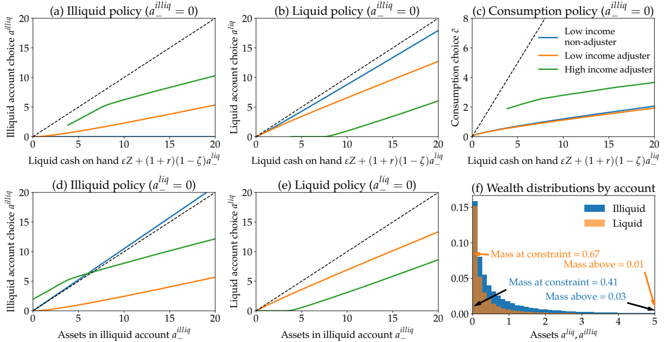
Figure D.3: Policies and distributions for calibrated HA-two model
