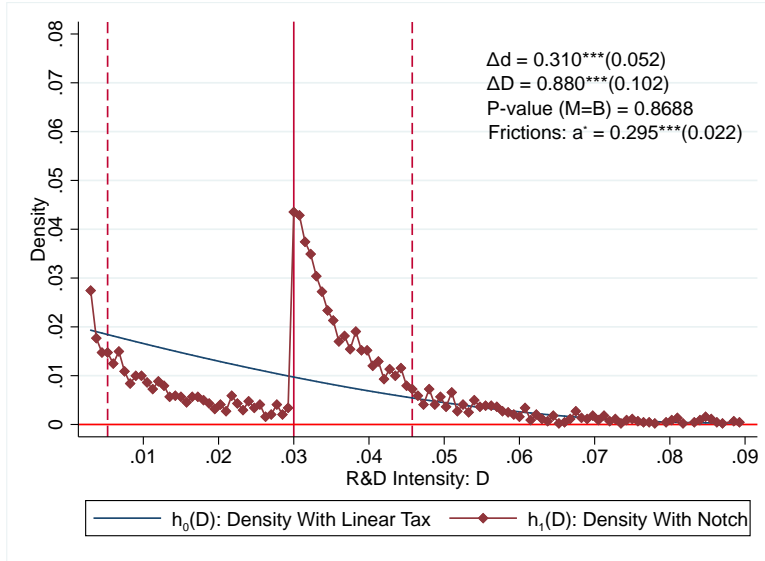
Figure A.6: Robustness of Bunching Estimates
