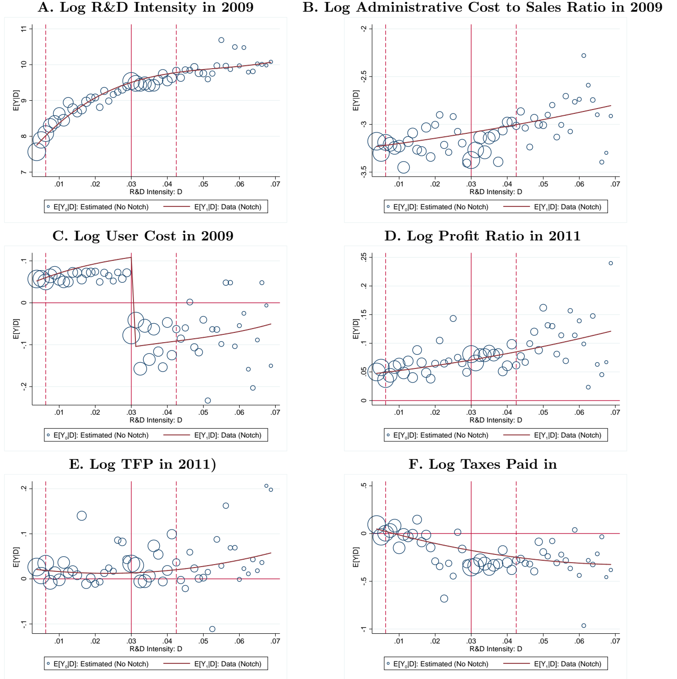
Figure A.7: Estimated Values of E[Y|d] for ITT Analysis
