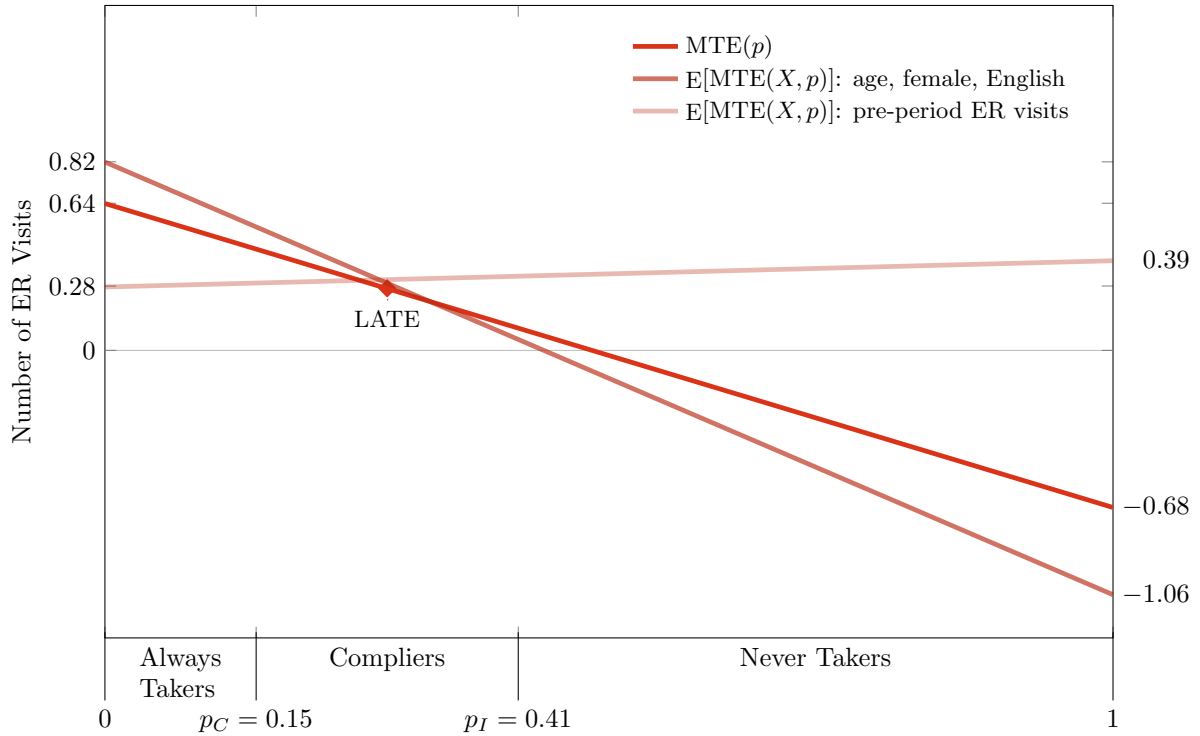
Figure 7: MTE(x, p) with Previous ER Utilization vs. MTE(x, p) with Common Observables
