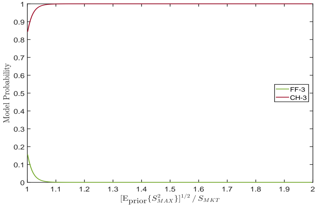
Figure A.1. Model probabilities comparing model CH-3 to model FF-3 The figure displays Bayesian posterior model probabilities for the two-way model comparison. The value on the horizontal axis is the square root of the prior expected maximum Sharpe ratio achievable by combining the model’s factors, divided by the observed Sharpe ratio of the market. Prior model probabilities are equal. The sample period is from January 2000 through December 2016 (204 months)
