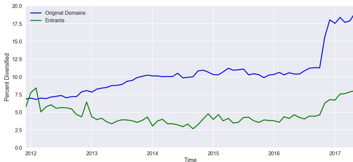
Figure 14: DNS diversification rates among original and entrant domains
