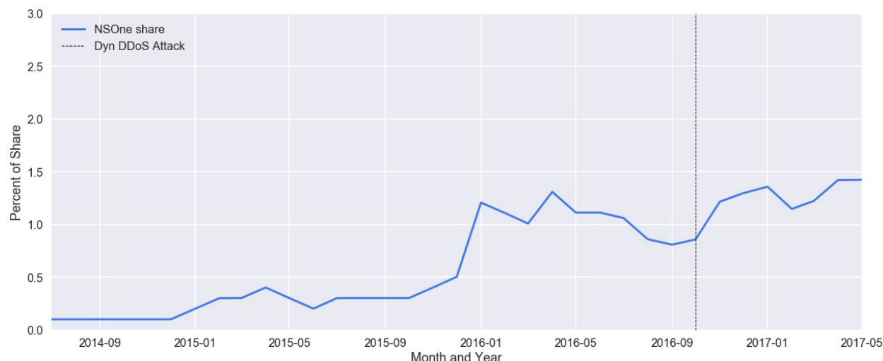
Figure 19: NSOne's market share of the DNS space before and after the Dyn attack
