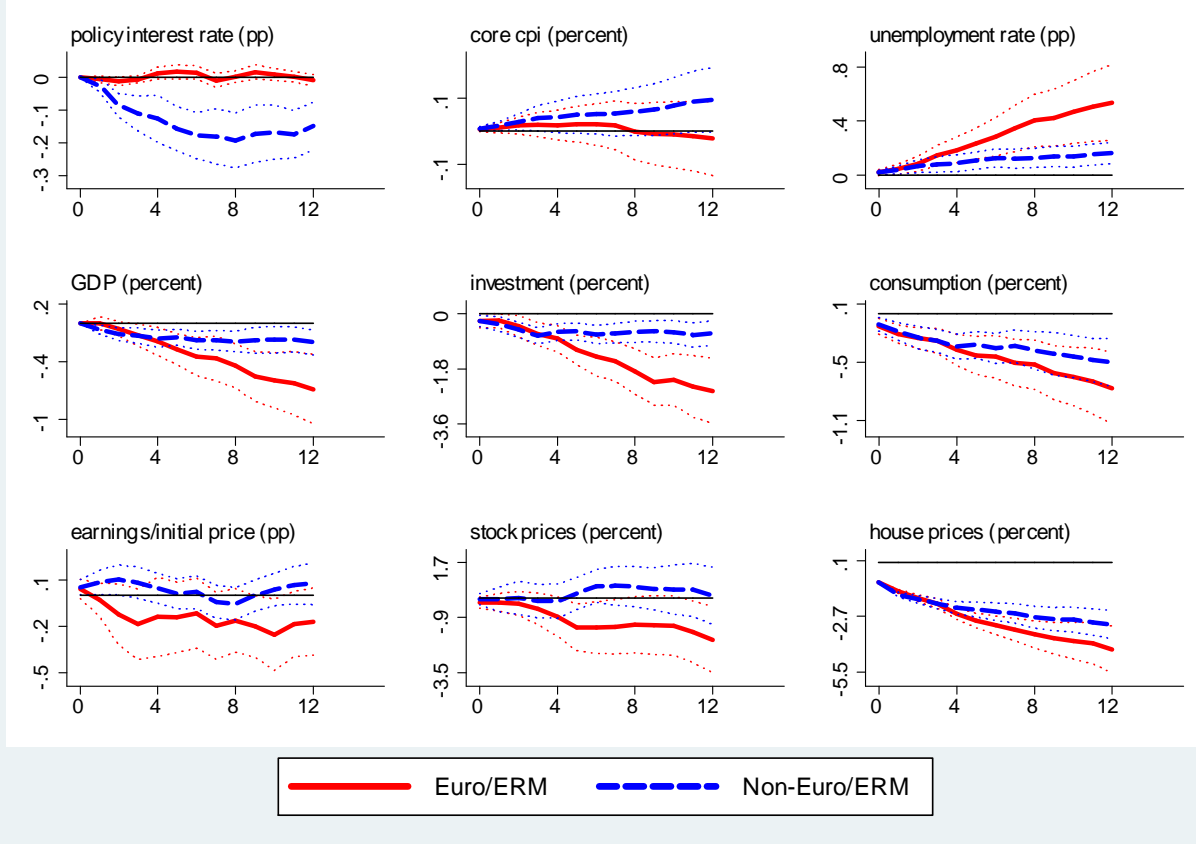
Figure 6: Results from the regression specification in (52) with the addition of the indicator variables for Euro/ERM and non-Euro/ERM status as well as the interaction of all right-hand-side variables with these indicators. The solid red (resp. dashed blue) lines plot the coefficients corresponding to the the negative log house price variable when the Euro/ERM status is equal to 1 (resp. 0). For the units, “percent” corresponds to 0.01 log units (i.e., it is approximate) and “pp” corresponds to percentage points. All regressions include time and country fixed effects; contemporaneous value and 12 lags of the first difference of log GDP; contemporaneous value and 12 lags of the policy interest rate; 12 lags of the first difference of log house prices; 12 lags of the first difference of the outcome variable. The dotted lines show 95% confidence intervals calculated according to Newey-West standard errors with a bandwidth of 20 quarters. All regressions are weighted by countries’ PPP-adjusted GDP in 1990. Data is unbalanced quarterly panel that spans 1990Q1-2017Q4. All variables except for those in the top panel are adjusted for inflation. Earnings are normalized by the stock price at the quarter before the shock (see Footnote 24). The sources and the definitions of variables are described in Appendix E.
