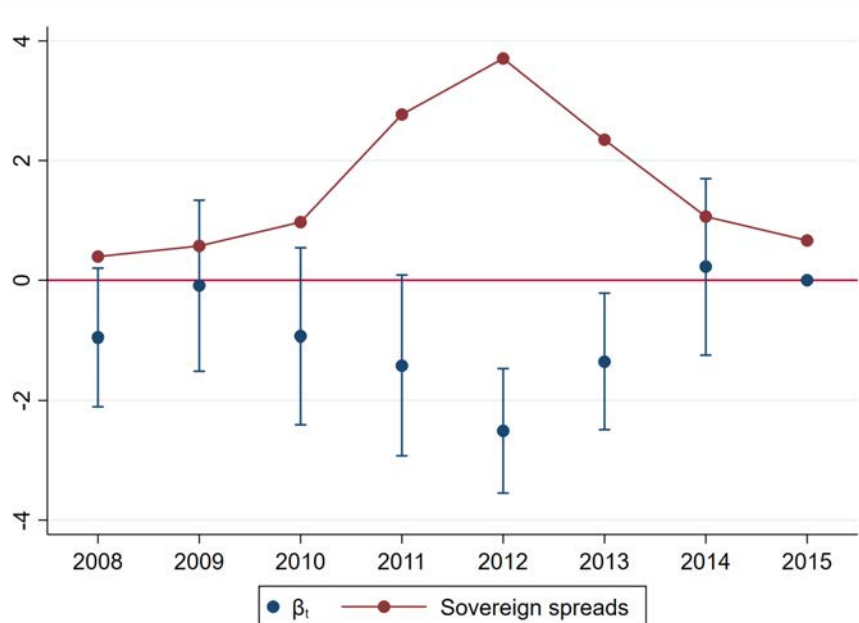
Figure 3: Estimation of \beta_t in equation (30)
