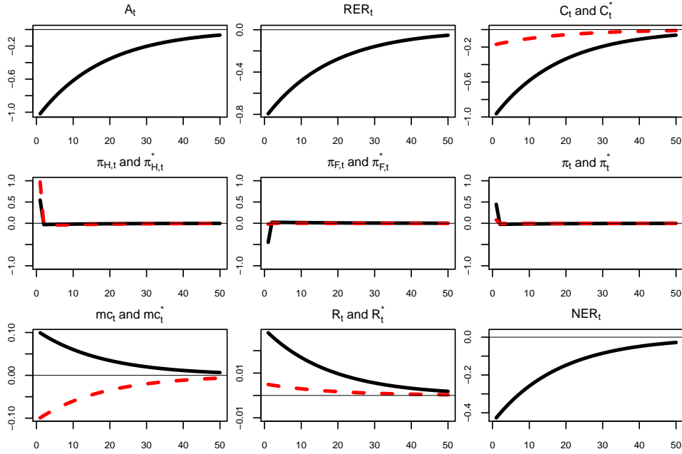
Figure 3: Response to technology shock under money-growth rule
