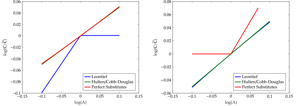
(a) log GDP with no reallocation/extreme decreasing returns. Perfect substitutes and Hulten's approximation overlap almost perfectly. (b) log GDP with full reallocation/constant returns. Leontief and Hulten's approximation overlap almost perfectly.
