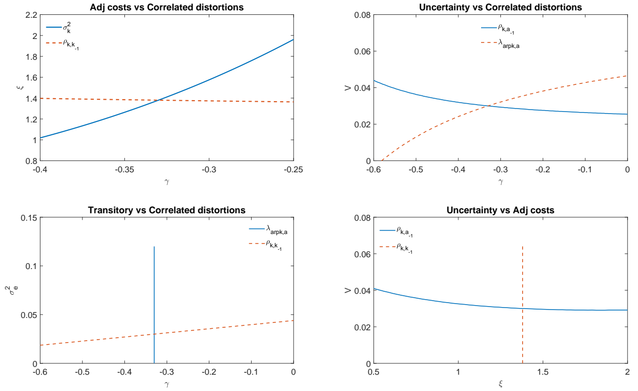
Figure 1: Pairwise Identification - Isomoment Curves
